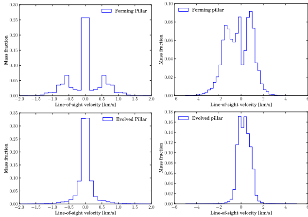
Fig. 14. Distribution of the gas mass as a function of the line-of-sight velocity for the snapshots in Fig. 13. Top : the spectra are taken when the pillar is forming and the shell collapsed, just before the shell has collapsed in on itself. The blue- and red-shifted components can be clearly identified in both cases and are associated with the curved shell. Bottom : after the collapse, when the pillar is in its growing state, the spectra display a single peak.
