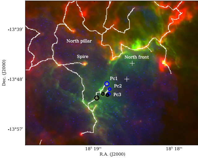
Fig. 9. Three-colour image of the interface between the Eagle Nebula and the H II region around NGC 6611 (red: Herschel column density map, green: PACS 70 \mu m, blue: H\alpha ). The white crosses indicate the O stars. Each spectrum in Fig. 10 is integrated inside the corresponding coloured circle.
