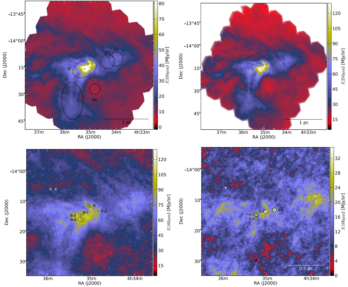
Fig. 2. Herschel intensity maps showing the areas used in the analysis. The maps show the total intensity after zero-point correction. (Top left) 350 \mu\text{m} (26.8'' resolution) showing the larger regions (A1, A2, B and C) and the background area (BG) used in the analysis. (Top right) 250 \mu\text{m} (18.3'' resolution) map showing the striation in L1642. (Bottom left) 160 \mu\text{m} (18.3'' resolution) showing the most prominent clumps identified by Getsources. FWHM ellipses of the clumps are drawn in the figure. (Bottom right) 100 \mu\text{m} (18.3'' resolution) showing the circular apertures (with 80'' diameter) used in the aperture photometry of the point sources marked in the figure.
