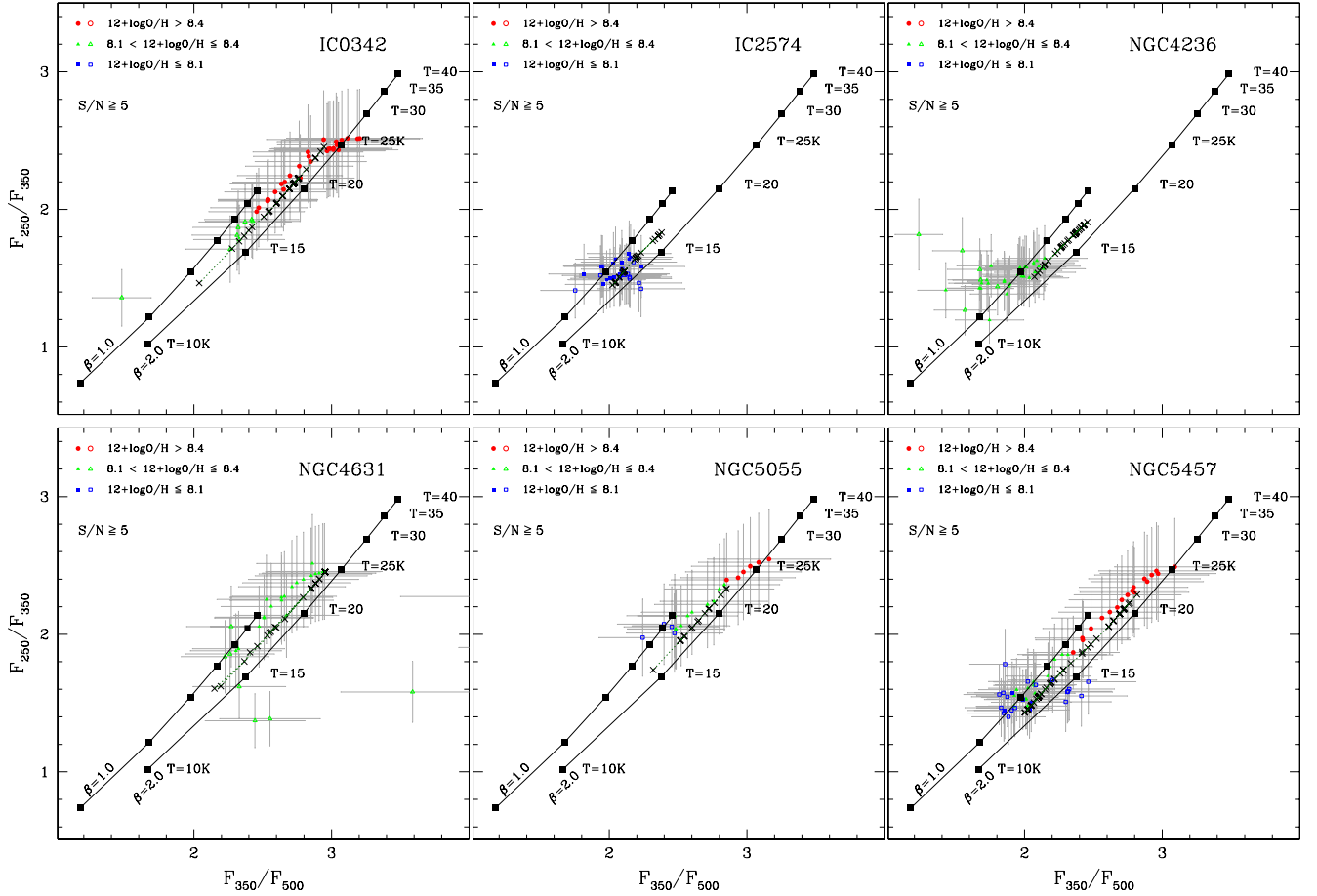
Fig. 6. SPIRE colors of individual galaxies with more than 30 radial data points. Data are distinguished by O/H with (red) circles showing 12 + \log(O/H) > 8.4 , (green) triangles 8.1 < 12 + \log(O/H) \leq 8.4 , and (blue) squares 12 + \log(O/H) \leq 8.1 . Filled symbols correspond to positions with normalized (to optical radius R_{opt} ) radii within R/R_{opt} \leq 0.8 , and open symbols to larger radii. DL07 best-fit models for the data are shown with \times , connected by a dotted line. In all panels, MBB fits are given for two values of emissivity index \beta : \beta = 1.0 (dotted line) and \beta = 2.0 (solid line). Temperatures are also labeled from T_{dust} = 15 K to T_{dust} = 40 K.
