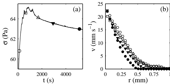
FIG. 1: Flow behavior in a rough Couette cell after a constant shear rate \dot{\gamma} = 25\text{ s}^{-1} is imposed at t = 0\text{ s} . (a) Stress response \sigma vs time t . (b) Velocity profiles v(r) at t = 123\text{ s} ( \circ ), 653\text{ s} ( \square ), 1702\text{ s} ( \Delta ), 2931\text{ s} ( \blacktriangledown ), and 5137\text{ s} ( \bullet ). r is the radial distance from the inner rotating cylinder. Error bars are of the order of the marker size.
