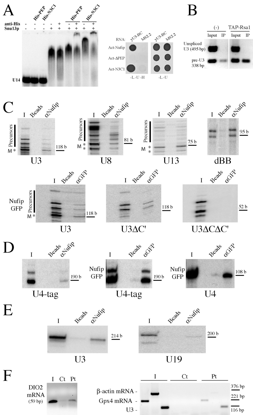
Figure 3. Nufip binds box C/D and H/ACA snoRNAs, a B/C-containing RNA, U4 snoRNA, and mRNAs coding for selenoproteins. (A) In vitro interactions of Rsa1 and Nufip with Snu13-RNA complexes. (left) Gel-shift assays show that the Rsa1 N3C1 and PEP domains interact with Snu13 bound to RNA. Radiolabeled yeast U14 snoRNA was incubated with the indicated recombinant proteins and anti-His antibodies when indicated. (right) Y3H assays show that Nufip interacts with yU3-B/C RNA in a PEP-dependent manner. Plate -Leu -Ura (-L -U) shows the growth of the test strain. Growth on -Leu -Ura -His (-L -U -H)
