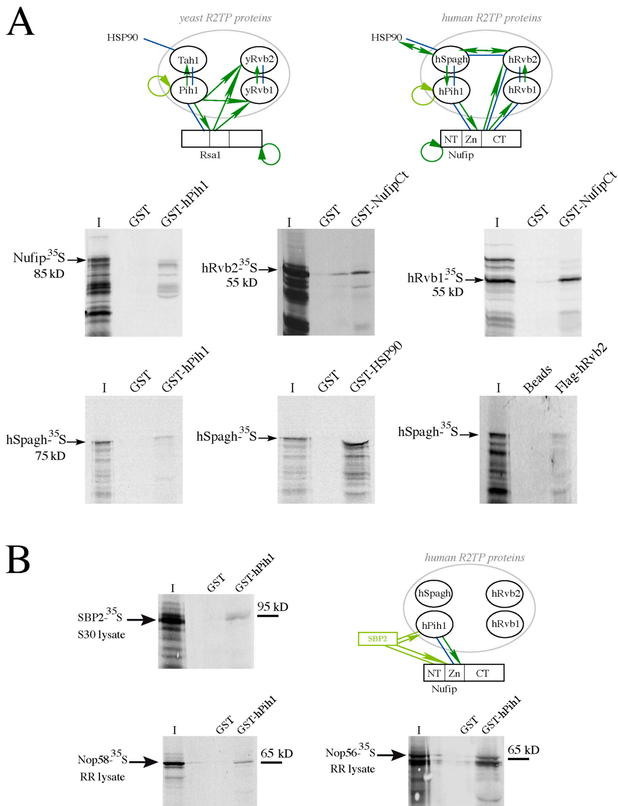
Figure 8. hSpagh, hPih1, and Nufip mediate the interaction of Hsp90 with hNop58, 15.5K, hNHP2, and SBP2. (A) Interactions between Rsa1, Nufip, and R2TP proteins. (top) Summary of interactions between yeast (left) and human (right) proteins. Y2H interactions are indicated by green arrows, and physical interactions observed in GST pull-downs are indicated by blue lines. (bottom) GST pull-down experiments. Legend as in Fig. 4. For the interaction between hSpagh and hRvb2, a FLAG-hRvb2 fusion was used. (B) SBP2, hNop56, and hNop58 interact with hPih1 in GST pull-down experiments. Legend as in A except that hNop56 and hNop58 were translated in rabbit reticulocyte lysates (RR). The schematic summarizes the interactions of SBP2 with Nufip and R2TP proteins (legend as in A).
