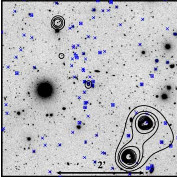
Figure 14. X-ray contours overlaid on an I -band image of the central region of the Cl1040–1155 field. The crosses indicate sources for which spectra have been obtained; the squares indicate spectroscopically confirmed cluster members. North is up and east is to the left-hand side.
