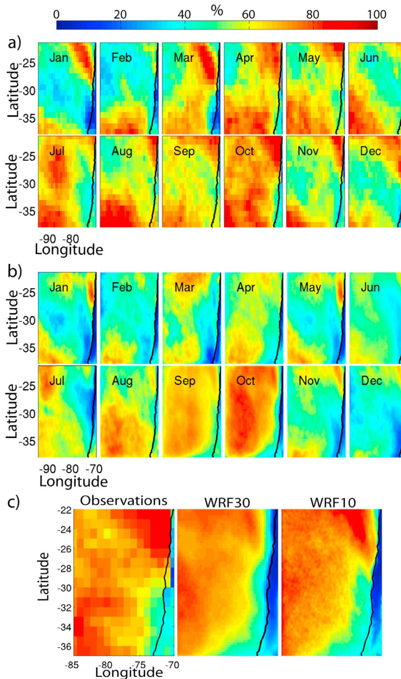
Figure 8. Monthly cloud-cover (in %) during year 2000 (a) from GOES-8 observations; (b) from WRF30; and (c) October only with additional results from WRF10.
