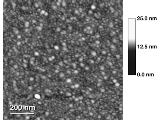
Fig. 2. Atomic force micrograph of 100 nm thick film deposited with 5 W bias power.
