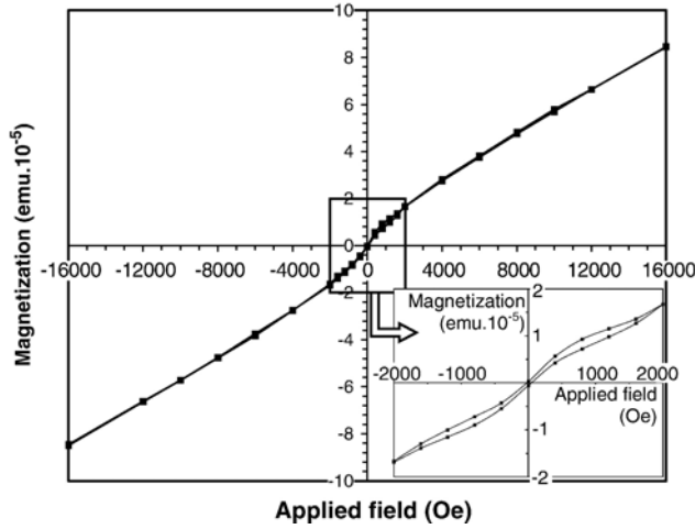
Fig. 3. In-plane magnetic hysteresis curve of a 300 nm thick film deposited with 5 W bias power, on both sides of a 4.5 \times 4.5 \times 0.15 mm 3 glass substrate.
