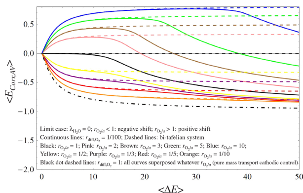
Figure 4. Similar curves to Figure 3, but r_{\text{diff,O}_2} = 0.01 . The curves for various r_{\text{O}_2/a} are represented as Figure 3. The dot-dashed curve at the most bottom position represents r_{\text{diff,O}_2} = 1 (cathodic kinetics entirely controlled by the diffusion).
