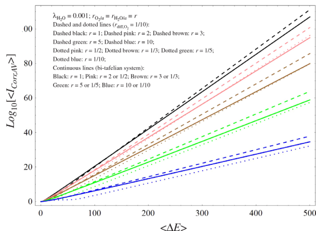
Figure 9. Enhancement of the corrosion current density; the same simulation conditions as in Figure 7, but with \lambda_{\text{H}_2\text{O}} = 0.001 .
