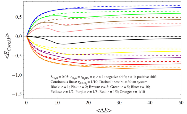
Figure 6. Effect of r_{\text{O}_2/\text{a}} (or r_{\text{H}_2\text{O}/\text{a}} ), and \langle E_{\text{corr},\text{AV}} \rangle with respect to \langle \Delta E \rangle , for a three reaction corrosion mechanism. The water reduction contribution to the total cathodic faradaic current is minor ( \lambda_{\text{H}_2\text{O}} = 0.05 ), and the oxygen reduction reaction is characterised by a small diffusion contribution ( r_{\text{diff},\text{O}_2} = 0.1 ) at E_{\text{corr},0} . Electrolyte resistance R_e is neglected. Comparison with a bi-Tafelian corrosion mechanism is shown as dashed lines. The Tafel constant ratio r supplies different curves, which are distinguished as indicated in Figure 3.
