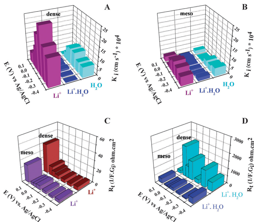
Fig. 10 Evolution of kinetic parameters, K_i , for a dense (A) and mesoporous (B) \text{WO}_3 thin films, and the comparative curve of the transfer resistance values ( R_{ti} = 1/F \cdot G_i ( \Omega \cdot \text{cm}^2 )) for cationic species in dense and mesoporous \text{WO}_3 thin films, \text{Li}^+ ions (C), and \text{Li}^+\cdot\text{H}_2\text{O} ions (D), presented as a function of applied potential.
