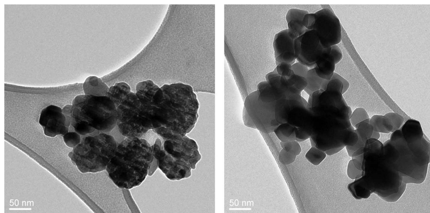
Figure 1. TEM images of commercial \text{TiO}_2 nanopowder mixture of rutile and anatase from Sigma Aldrich (a) and pure anatase from MK Impex Corp. (b).
