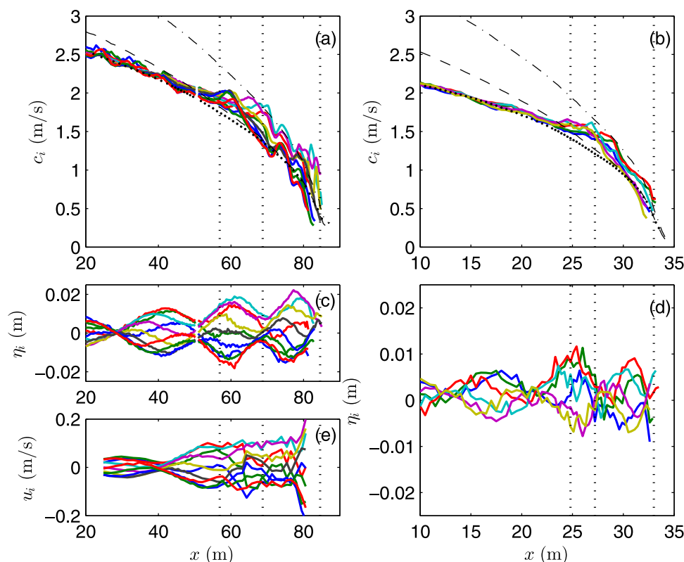
Figure 4. (a) Individual wave celerity, (c) infragravity-wave-induced variations of the water level \eta_i , and (e) velocity u_i ( u_i > 0 : onshore-directed current) for case G3. (b, d) Individual wave celerity and variations of water level for case A4 (too few velocity measurements for case A4). In Figures 4a and 4b, the black dots show linear celerity c_{lin} (equation (1)) calculated from the mean offshore period T_0 and the local mean water depth \bar{h} , the thin dashed line is (gh)^{1/2} and the dash-dotted line is 1.3(gh)^{1/2} . For a given case, each wave has a designated color (same colors as in Figure 2). See caption of Figure 1 for definition of the vertical dotted lines.
