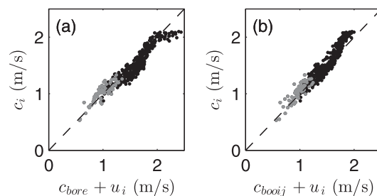
Figure 11. Individual wave celerity c_i in the surf zone as a function of (a) c_{bore} + u_i and (b) c_{booij} + u_i . Only data for which velocity measurements were available are shown (391 estimates, same data points as Figure 7). The gray dots correspond to shallowest water depth ( \bar{h} < 0.10 m, i.e., d^* \leq 1/3 ).
