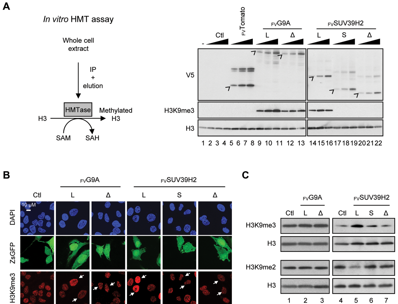
Figure 4. Inclusion of SUV39H2 exon 3 is required to encode an active histone methyltransferase. (A) In vitro analysis of the methyltransferase activity associated to each FvG9A and FvSUV39H2 isoforms. Scheme of the in vitro histone methyltransferase (HMT) assay procedure (left panel). Various quantities of purified FvG9A and FvSUV39H2 (right panel) were incubated with the recombinant human histone H3.1 and S-adenosylmethionine (SAM) producing methylated H3.1 and S-adenosylhomocysteine (SAH). Histone H3 and H3K9me3 were analyzed by western blot using specific antibodies (right panel). Control reactions were supplemented with FvTomato, water (-) or sample issued from blank purification procedure (Ctl). Levels of recombinant proteins were estimated using V5 antibody. (B) and (C) H3K9me3 was assessed in HeLa cells after expression of FvG9A and FvSUV39H2 isoforms. (B) DNA was counterstained with DAPI (blue), H3K9me3 was immunostained with a specific antibody (red) and cells expressing FvG9A and FvSUV39H2 were revealed with ZsGreen1 Fluorescence Protein (ZsGFP panel; labeled with white arrows in H3K9me3 panel). (C) Analysis of H3K9me3, H3K9me2 and H3 levels by western blot in total protein extracts of HeLa cells expressing FvG9A and FvSUV39H2 isoforms.
