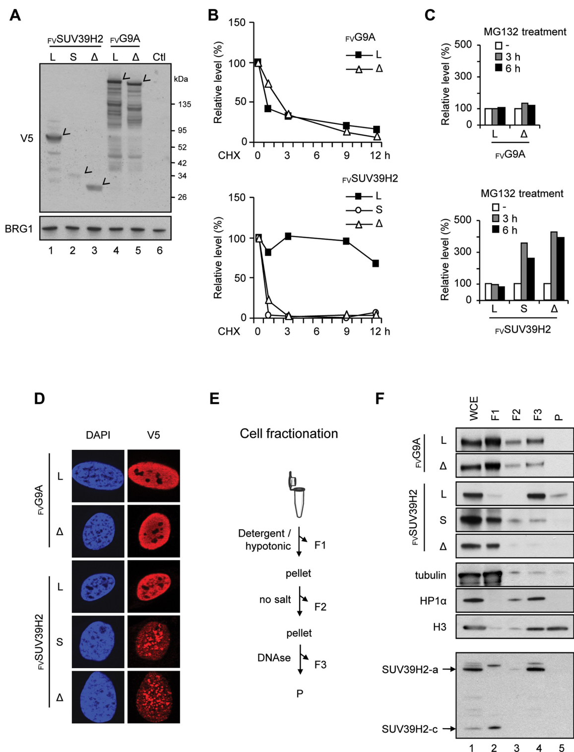
Figure 3. Protein stability and sub-nuclear localization of SUV39H2 isoforms are regulated by alternative inclusion of exon 3. (A) Expression in HEK 293T cells of ectopic tagged G9A and SUV39H2 protein isoforms. Cells were transfected with the pLVX vector containing Flag-V5 tags and SUV39H2 or G9A cDNA to express exogenous protein isoforms (FvSUV39H2 or FvG9A). Cells transfected with pLVX empty vector were used as controls (Ctl). The ectopic proteins were revealed by western blot using the V5 antibody. (B) and (C) Stability analysis of each G9A and SUV39H2 protein isoform. FvG9A and FvSUV39H2 isoforms were assessed by western blot in HeLa cells treated with cycloheximide (CHX) (B) or MG132 (C) for the indicated times in hours (h). The signal detected with V5 antibody was normalized to histone H3 levels. (D) Localization of FvG9A and FvSUV39H2 isoforms in HeLa cells. Exogenous proteins were revealed with V5 antibody (red), while DNA was counterstained with DAPI (blue). (E) and (F) Analysis of FvG9A and FvSUV39H2 and the endogenous SUV39H2 isoforms after fractionation of HeLa cells. (E) Scheme displaying the cell fractionation procedure. (F) Protein isoforms were detected in whole cell extracts (WCE) and fractions by western blot using the V5 or SUV39H2 antibodies. Endogenous tubulin, HP1α and H3 proteins were analyzed as markers of the cell fractions.
