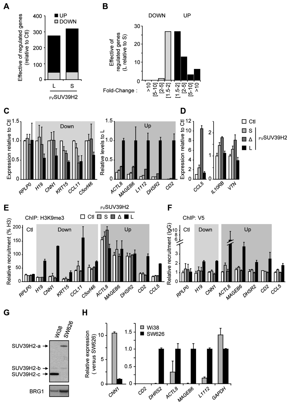
Figure 5. Alternative inclusion of SUV39H2 exon 3 modulates the expression of target genes. (A) Graph showing the number of genes that are up- or down-regulated in HeLa cells expressing FVSUV39H2-L or FVSUV39H2-S. Gene expression levels were assessed by high throughput RNA sequencing and hits were retained with a threshold of 1.5 fold-change ( P -value < 0.05) when compared to control (Ctl, virus generated with empty construct). (B) Graph displaying the differential effect on gene expression of FVSUV39H2-L versus FVSUV39H2-S. Number of genes is displayed in function of expression fold change. (C and D) Validation of 13 genes differentially affected in their transcription by SUV39H2 isoforms. Transcription levels were analyzed by RT-qPCR and quantification was displayed as means \pm s.e.m. of three experimental replicate. (C) Five genes down-regulated by the over-expression of FVSUV39H2-L (Down) were shown relative to control (Ctl). RPLP0 gene is shown as unaffected gene. Five genes up-regulated by the over-expression of FVSUV39H2-L (Up) were presented relative to the expression in presence of FVSUV39H2-L (set to 1). (D) Expression analysis of three genes up-regulated specifically by FVSUV39H2-S and \Delta isoforms. Transcriptional levels were expressed relative to control (Ctl). (E and F) Analysis of H3K9me3 and SUV39H2 isoforms at promoters of target genes. Chromatin from cells expressing FVSUV39H2 isoforms or not (Ctl) was immunoprecipitated with antibodies to H3, H3K9me3, V5 tag or nonimmune (IgG). Relative enrichments were measured by qPCR using primer sets targeting promoters of indicated genes. Values are means \pm s.e.m. of three independent experiments. Amounts of H3K9me3 are expressed in percent of H3 (E), and amounts of FVSUV39H2 isoforms are expressed relatively to IgG control (F). (G) Endogenous SUV39H2 isoforms expressed in WI38 and SW626 cell lines were detected by western blot. (H) Relative gene expression in WI38 and SW626 cells of seven hits validated in panel 5C were quantified by RT-qPCR. CD2 gene expression is not detectable in both cell lines.
