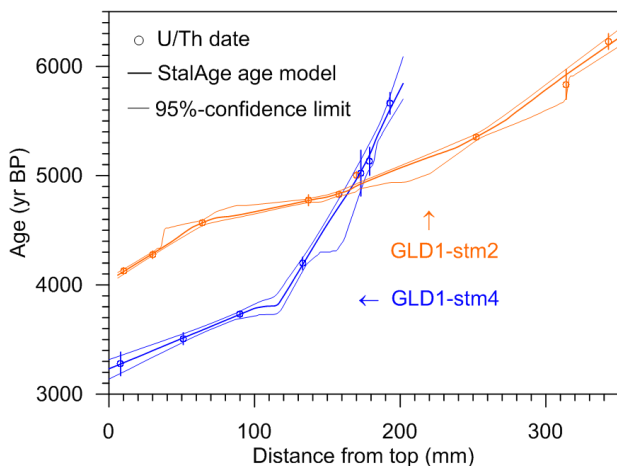
Figure 3. Age models of stalagmites GLD1-stm2 and GLD1-stm4 from the Gueldaman GLD1 Cave. The age models were calculated using the StalAge program (Scholz and Hoffmann, 2011). Note that the U/Th date of sample GLD1-stm4-47 was detected as a major outlier and not used in the final age model of stalagmite GLD1-stm4. The 2\sigma analytical uncertainty of each U/Th date (dot) is represented by the error bars, whereas the 95 % uncertainty assessed from the model simulation is represented by thin curves.
