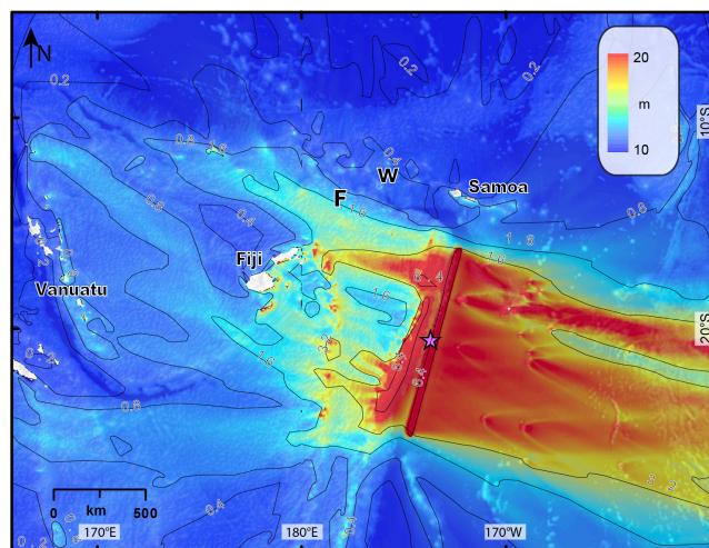
Figure 8. Tsunami maximum wave elevation (in m) generated by the full rupture of the Tonga Trench (Sc. 8, Table 4). Model generated using the Gerris flow solver. F: Futuna, W: Wallis. The star is the epicentre.
