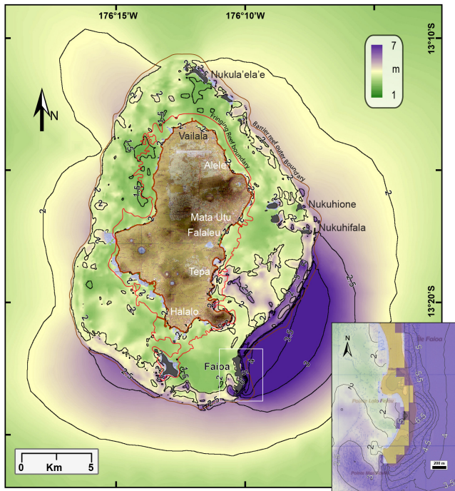
Figure 9. Maximum wave elevation (in m) at Wallis generated by an M_W = 9.1 earthquake along the Tonga Trench. Model generated using the Gerris flow solver. The outer boundary of the barrier reef (brown line) and the outer boundary of the fringing reef (red line) are from ReefBase database. Insert: enlargement on the reef island of Faioa.
