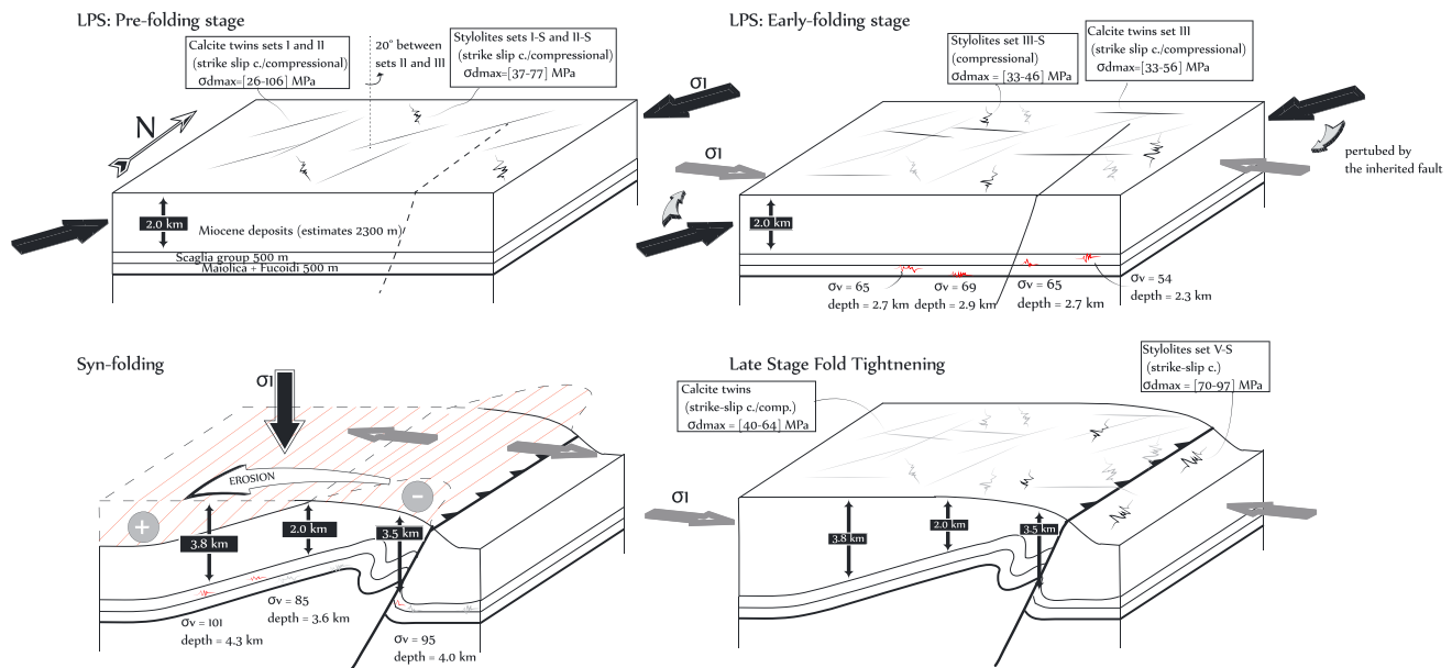
Figure 9. Interpretative sketch reporting the evolution of microstructure development, maximum burial evolution and stress history in the Monte Nero Anticline inferred from the whole data set including the stylolite roughness paleopiezometry. Note that only prefolding LPS and fold-related stages are represented. Drawing does not reflect microstructure distribution, abundance, or size.
