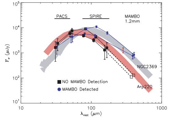
Figure 4. The far-IR part of the SED of two MAMBO-detected (blue circles) and two MAMBO-undetected sources (black squares) from our sample (divided by 1+z ). All four sources are chosen to have comparable L_{\text{IR}} and f_{250} . The far-IR part of the SED of Arp 220 (coral shaded area) and that of NGC 2369 (grey shaded area) are also shown. For the MAMBO-undetected sources the open boxes correspond to the 1.2-mm flux density based on the SED extrapolation. The red arrow indicates the confusion limit of 850- \mu\text{m} surveys. The SED of MAMBO-undetected sources peaks at shorter wavelengths, indicating warmer T_d and lower 850–1200 \mu\text{m} emission when compared to that of IRAM-detected sources. This plot illustrates that among sources with comparable L_{\text{IR}} those with higher T_d are missed by current ground-based surveys.
