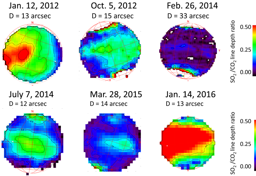
Fig. 8. Example maps of the line depth ratio of a weak \text{SO}_2 multiplet around 1345.11 \text{cm}^{-1} (7.4 \mu\text{m} ) divided by a weak \text{CO}_2 transition at 1345.22 \text{cm}^{-1} , recorded during each of the TEXES observing runs. The scale is the same for the six maps. The exact dates and durations of the maps are indicated in Table 2.
