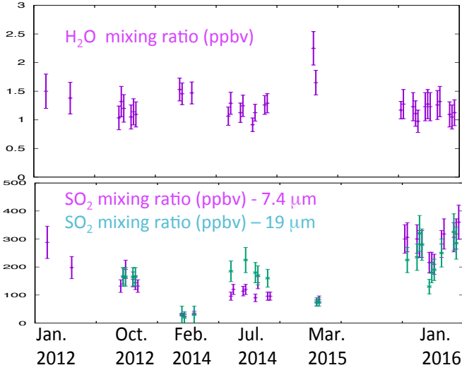
Fig. 21. Long-term variations of the \text{H}_2\text{O} volume mixing ratio ( top , measured at 7.4\ \mu\text{m} ) and the \text{SO}_2 volume mixing ratio ( bottom , measured at 7.4 and 19\ \mu\text{m} ) between January 2012 and January 2016. The January 2012 and March dataset correspond to evening terminator observations; the 4 other datasets correspond to morning terminator observations. All data were obtained using the lines listed in Table 3, with the exception of the first HDO measurement (January 10, 2012) and the two 19\text{-}\mu\text{m} \text{SO}_2 measurements of October 4, 2012, which were taken using different transitions (E12, E13). For the conversion from HDO to \text{H}_2\text{O} abundances on Venus, we assume a D/H ratio of 200 times the VSMOW (Fedorova et al. 2008).
