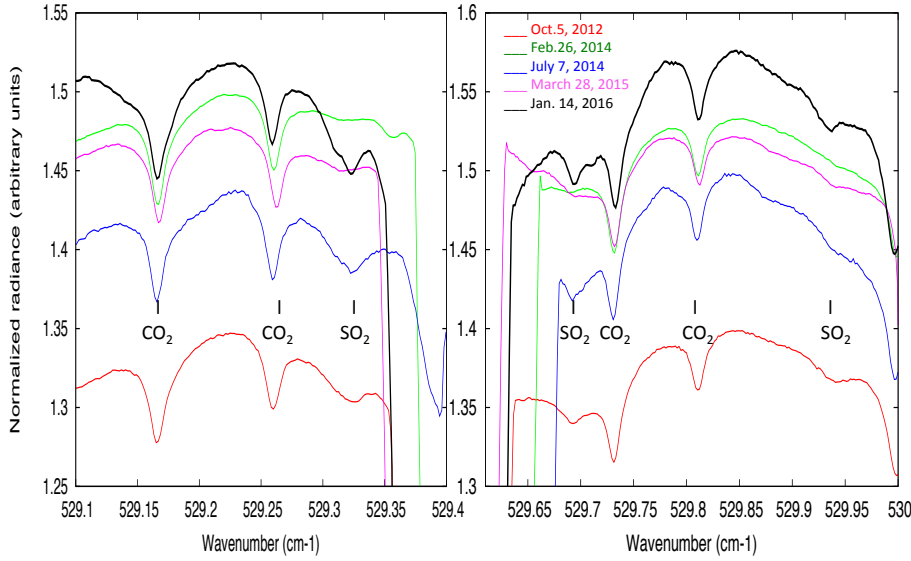
Fig. 7. Examples of disk-integrated spectra recorded during each of the TEXES observing runs in the 18.9- \mu m range. Left: 529.1–529.4 \text{cm}^{-1} ; right: 529.65–530 \text{cm}^{-1} . The exact dates and durations of the corresponding observations are indicated in Table 2. It can be seen that the \text{SO}_2 absorption bands are strongest in January 2016, and weakest in February 2014.
