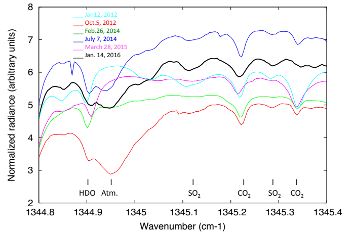
Fig. 6. Examples of disk-integrated spectra recorded during each of the TEXES observing runs between 1344.8 and 1345.4 \text{ cm}^{-1} ( 7.4 \mu\text{m} ). The exact dates and durations of the corresponding observations are indicated in Table 2. It can be seen that the SO 2 absorption bands are strongest in January 2016, and weakest in February 2014.
