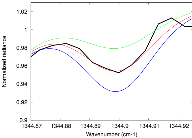
Fig. 20. Disk-integrated spectrum of the HDO transition at 1344.90 cm -1 recorded by TEXES on January 14, 2016 (20:33 UT). The date and duration of the corresponding observation are indicated in Table 2. The January 2016 run corresponds to the strongest SO 2 content measured at the cloudtop between 2012 and 2016. Thick black line: the TEXES data; thin lines: models. Green: H 2 O = 0.5 ppmv; red (best fit): H 2 O = 1.0 ppmv; blue: H 2 O = 1.5 ppmv. For the conversion between the HDO and H 2 O abundances on Venus, we assume a D/H ratio of 200 times the VSMOW (Fedorova et al. 2008).
