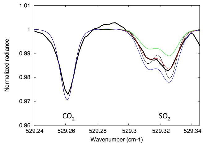
Fig. 16. Disk-integrated spectrum recorded by TEXES on January 14, 2016, between 529.24 and 529.345 cm -1 (19 μm), showing weak transitions of CO 2 and SO 2 . The date and duration of the corresponding observation are indicated in Table 2. The January 2016 run corresponds to the strongest SO 2 content measured at the clouddtop between 2012 and 2016. Thick black line: TEXES data; thin lines: models. Green: SO 2 = 200 ppbv with cutoff; red (best fit): SO 2 = 300 ppbv with cutoff; blue: SO 2 = 400 ppbv with cutoff; black: SO 2 = 65 ppbv, constant with altitude. The spectral resolution is 0.010 cm -1 .
