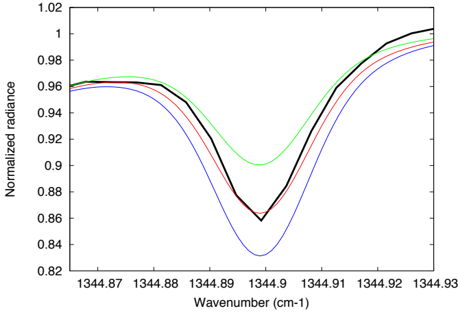
Fig. 19. Disk-integrated spectrum of the HDO transition at 1344.90 cm -1 recorded by TEXES on February 26, 2014, (7.4 μm). The dates and durations of the corresponding observation are indicated in Table 2. The February 2014 run corresponds to the weakest SO 2 content measured at the cloudtop between 2012 and 2016. Thick black line: the TEXES data; thin lines: models. Green: H 2 O = 1.0 ppmv; red (best fit): H 2 O = 1.5 ppmv; blue: H 2 O = 2.0 ppmv. For the conversion between the HDO and H 2 O abundances on Venus, we assume a D/H ratio of 200 times the VSMOW (Fedorova et al. 2008).
