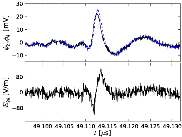
Fig. 9. Example of an ESW produced in the laboratory using the LAPD with an injected beam. Top panel: potentials as measured by two different probes separated by 80\text{ }\mu\text{m} with probe 2 (black) detecting the ESW slightly earlier than Probe 4 (blue). Bottom panel: the electric field calculated as the difference of the two potentials divided by the probe separation.
