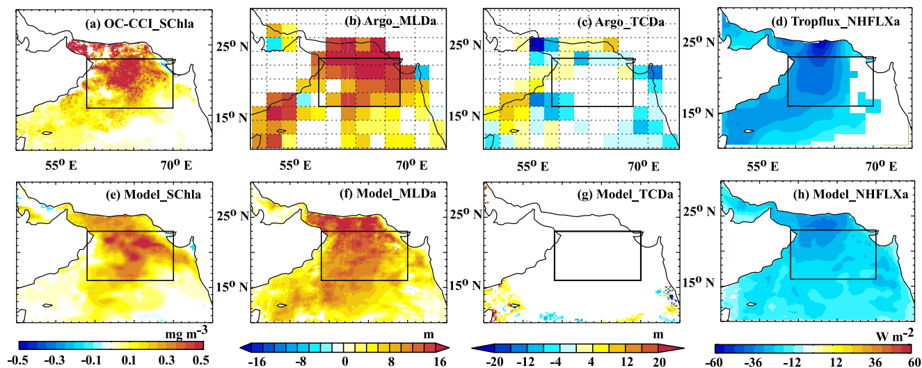
Figure 10. Observed interannual anomalies of (a) SCHl (OC-CCI), (b) MLD, (c) TCD (Argo-derived), and (d) net surface heat flux (TropFlux) for composite SCHl blooms (built from half of the difference between positive and negative events highlighted in Fig. 8). The SCHl composites are built from the months of max SCHl anomaly: March 2003, March 2008, and March 2012 for positive events; March 2007, March 2009, and February 2013 for negative events. The MLD and TCD composites are built from the months of February of the same year. (e–h) Idem for the model. For the model, composites are built from the positive and negative events highlighted in Fig. 7 (SCHl is composited using March 1995, 2000, 2008, and 2012 and February 2001 for positive events and March 1999, 2004, 2006, 2007, and 2009 for negative events; MLD and TCD are composited using February of the same years). Regions where composite values are less than the standard error are displayed in white.
