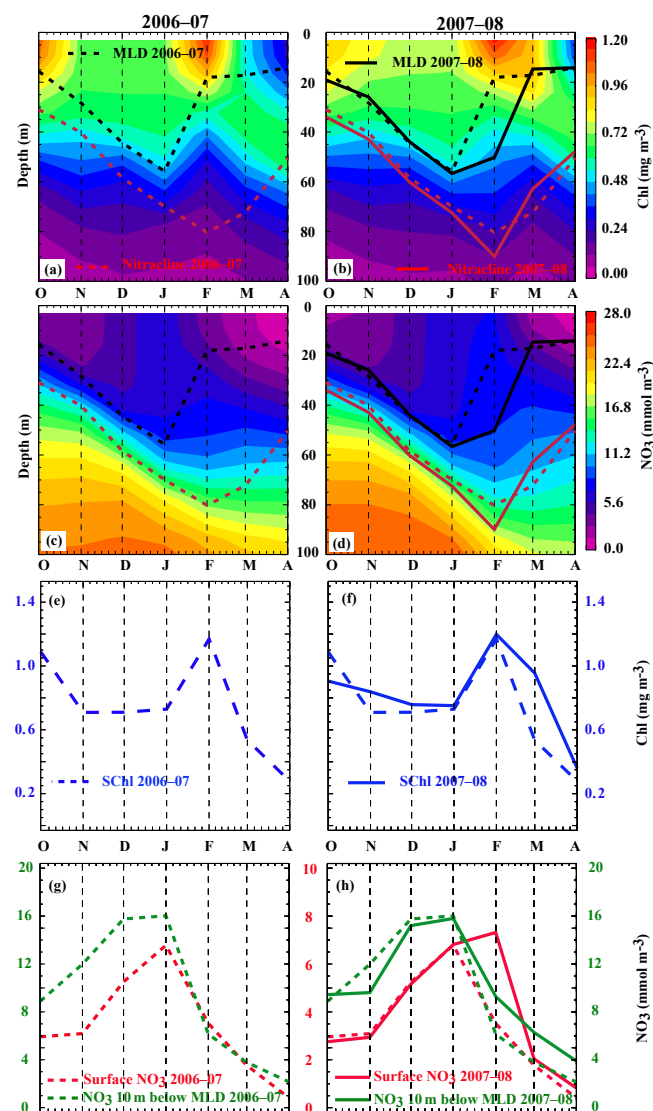
Figure 11. Depth–time section of NAS-averaged (a, b) chlorophyll (Chl) and (c, d) nitrate ( \text{NO}_3 ) for (a, c) 2006–2007 and (b, d) 2007–2008. The black lines indicate the MLD, thick for 2007–2008 and dashed for 2006–2007. The red lines similarly indicate the nitracline depth. Time series of NAS-averaged (e, f) SChl (blue curve) and (g, h) surface nitrate (red curve) and nitrate concentration 10m below the bottom of the MLD (green curve) for (e, g) 2006–2007 and (f, h) 2007–2008. In (f, h), the 2006–2007 values have been reported as dashed curves to ease comparisons between the two years.
