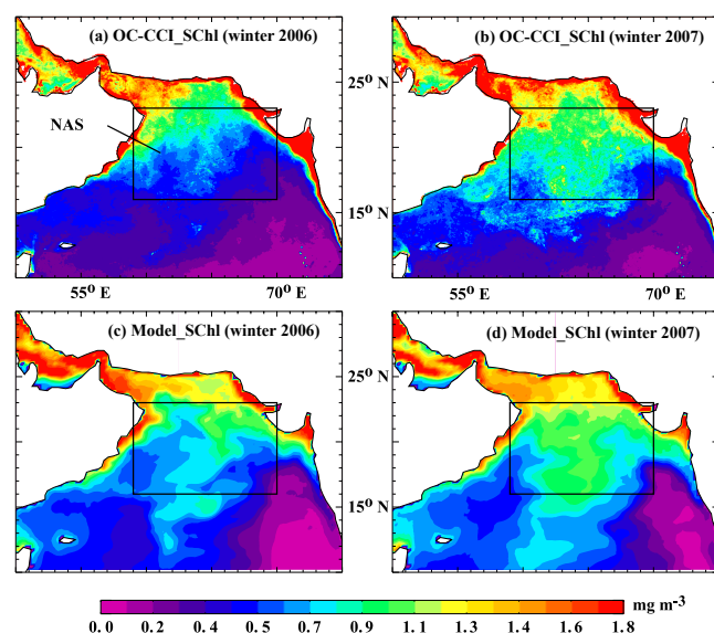
Figure 1. Arabian Sea average Schl for the winter (DJFM) of (a, c) 2006 and (b, d) 2007 in (a, b) OC-CCI product and (c, d) model. The NAS (North Arabian Sea) box (59–70° E, 16–23° N) is indicated by a black frame for future reference.
