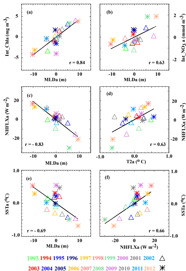
Figure 12. Scatter plot of modelled interannual NAS-box-averaged winter (February–March) anomalies of (a) 0–200 m total chlorophyll content against MLD. (b) Average MLD nitrate vs. MLD. (c) Surface net heat flux vs. MLD. (d) Surface net heat flux vs. 2 m air temperature. (e) SST vs. MLD. (f) SST vs. surface net heat flux. Plain lines indicate regression coefficients that are significantly different from zero at the 90 % confidence level.
