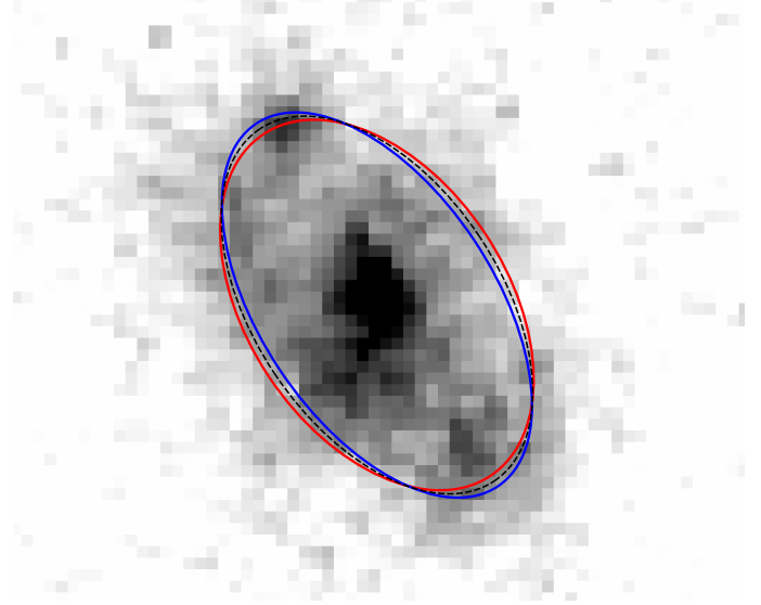
Fig. A.2. Example of the ellipse that overlaps the HST/ACS image with b/a as measured in the Zurich Structure and Morphology Catalog (black dashed ellipse) and as it appears using the lower (red solid ellipse) and upper (blue solid ellipse) value of b/a measured in Eq. (A.1).
