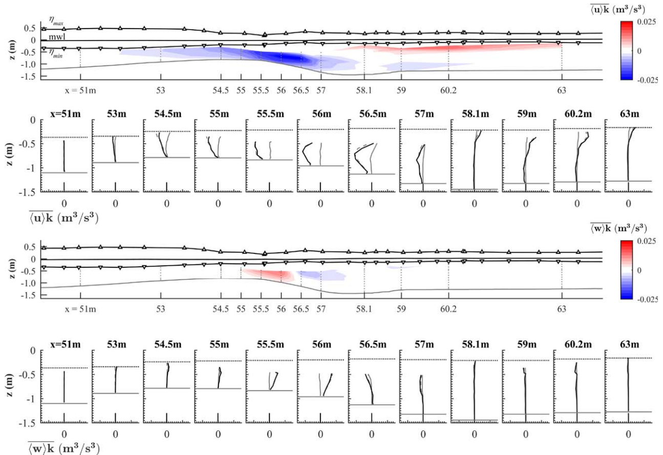
Figure 14. Time-averaged advection of turbulent kinetic energy: (top) \overline{\langle u \rangle k} and (bottom) \overline{\langle w \rangle k} . The gray profiles represent the wave-related (solid) and current-related (dashed) transport component.
