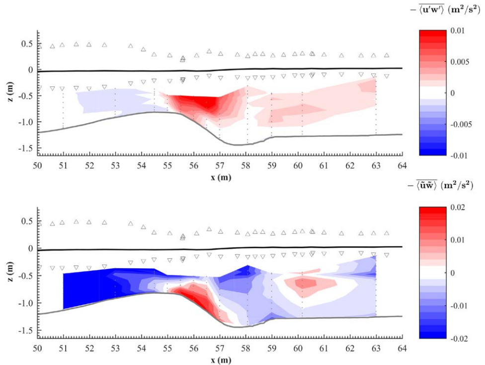
Figure 13. (top) Time-averaged turbulent Reynolds shear stress -\langle u'w' \rangle and (bottom) time-averaged wave Reynolds stress -\langle \bar{u}\bar{w} \rangle . The dots indicate the measurement locations; triangles indicate the maximum (crest) and minimum (trough) water surface elevation.
