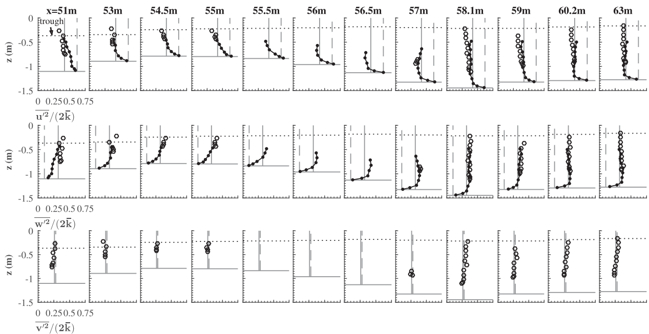
Figure 10. Ratios of time-averaged turbulence intensities. The gray vertical lines indicate Svendsen's [1987] ratios for surf zone turbulence: \bar{u}^2/2\bar{k} = 0.42 , \bar{w}^2/2\bar{k} = 0.32 , \bar{v}^2/2\bar{k} = 0.26 and the dashed lines Townsend's [1976] ratios for inner boundary layer turbulence: 0.62 : 0.10 : 0.28 .
