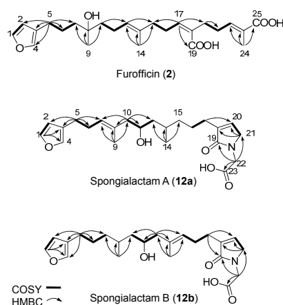
Figure 5. Selected COSY and HMBC correlations for compounds 2 , 12a and 12b .
