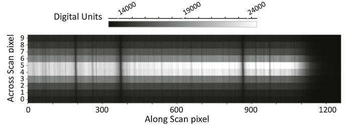
Fig. 15. Early RVS spectrum: Class 0 window ( 12.6 \times 0.3 mm on the CCD) of the G_{\text{RVS}} = 6.2 star with transit_ID=4635432253571710_1 from telescope 1 in FPA Strip 15, Row 4, observed on 2014 January 23. In this raw image, the bias level has not been subtracted and the aspect ratio of the window is widened in the across-scan direction for better visibility. The grey-scale is linear in digital units ( \sim 0.55 e - ).
