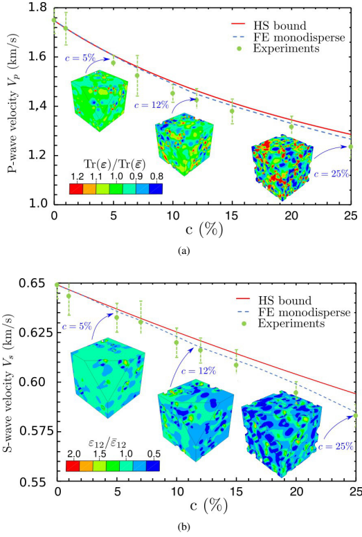
Figure 3: Effective (a) P-wave velocity V_p , (b) S-wave velocity V_s of microstructures with spherical single-size voids as a function of the porosity c . Comparison between the analytical HS bounds, FE monodisperse numerical estimates and experimental results.
