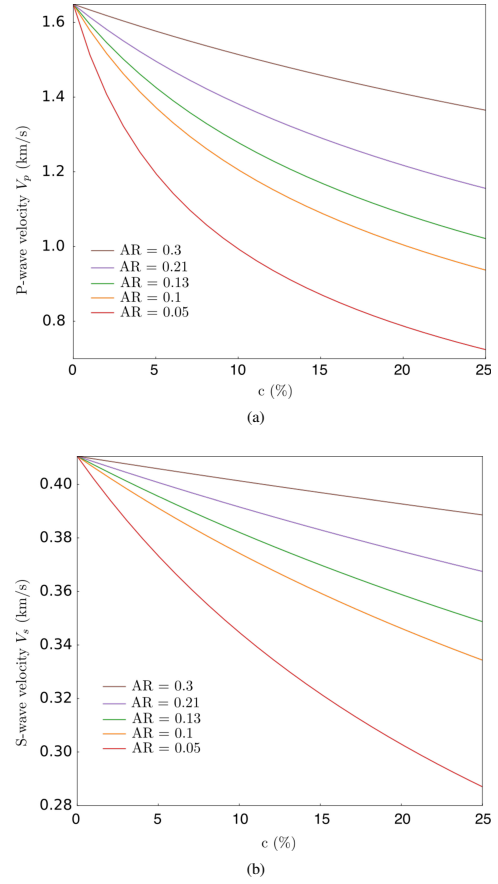
Figure 7: Results of :a) P-wave velocity b) S-wave velocity, variations due to change in the aspect ratio of the ellipsoidal voids.
