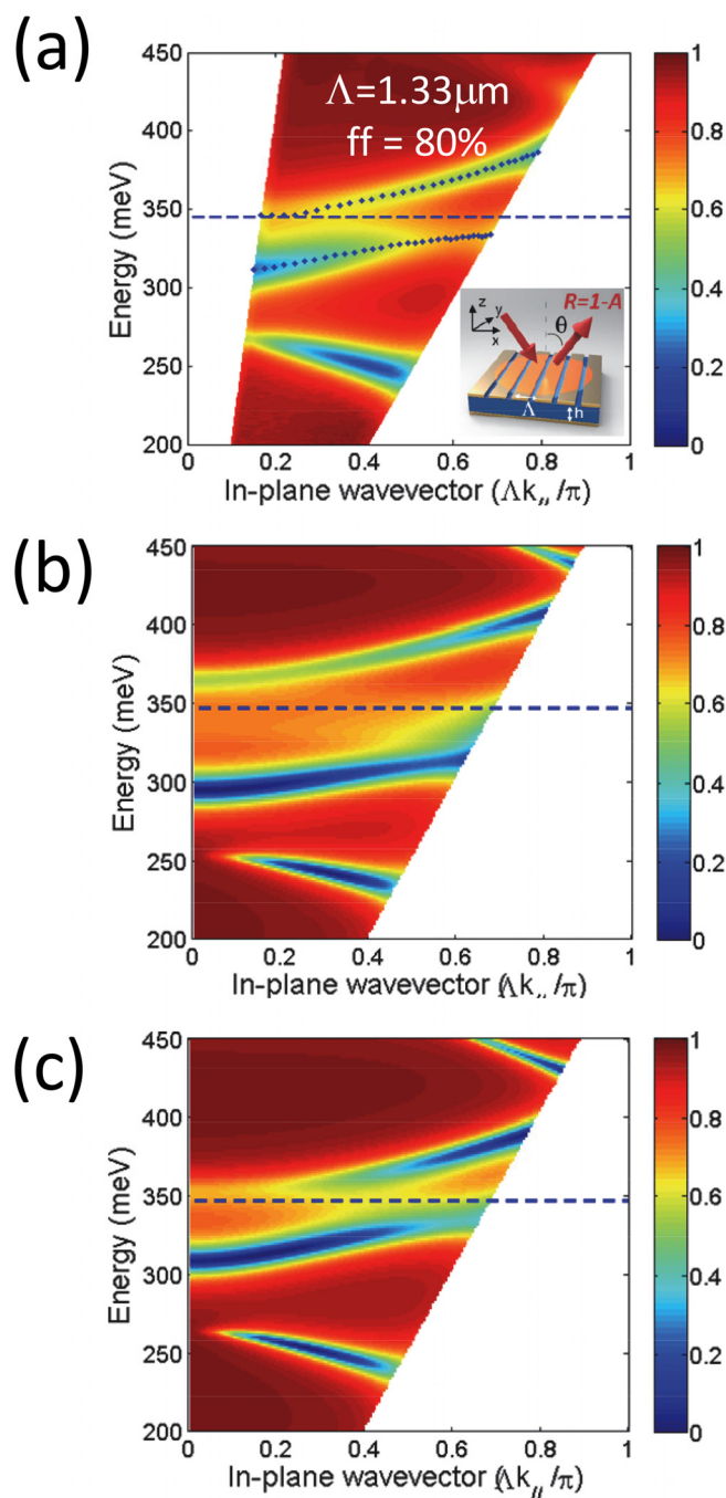
FIG. 3. (a) Experimental polaritonic dispersion of sample C231. The measurement geometry is reported in the inset, and more details can be found in Ref. 20. The lowest incidence angle is 13^\circ , while the highest is 73^\circ . The grating period is 1330 nm and the filling factor ( ff ) is 80%. The grating was fabricated by electron beam lithography, followed by deposition of Ti/Au layers. The polariton peaks are marked by dots, while the bare ISB transition corresponds to the dashed horizontal line. A Rabi splitting of approx. 36 meV is obtained. (b) Calculated polaritonic dispersion of sample C231 without taking into account non-parabolicity effects: the Rabi splitting is largely over-estimated. (c) Calculated polaritonic dispersion with the inclusion of the non-parabolicity effects: the agreement with the experiments is excellent.
