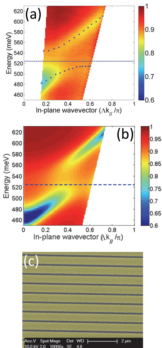
FIG. 4. (a) Experimental polaritonic dispersion of sample EQ247. The measurement geometry is similar to the previous sample. The grating period is 790 nm and ff is 93%. The polariton peaks are marked by dots, while the estimated ISB transition corresponds to the dashed horizontal line. For an estimated ISB wavelength of 2.32 \mu\text{m} , the longest wavelength attained by the lower-polariton is 2.58 \mu\text{m} , while the shortest wavelength (upper polariton) is 2.03 \mu\text{m} . (b) Calculated polaritonic dispersion with the inclusion of the non-parabolicity effects: the agreement with the experiments is excellent. (c) Colored SEM image of a typical grating.
