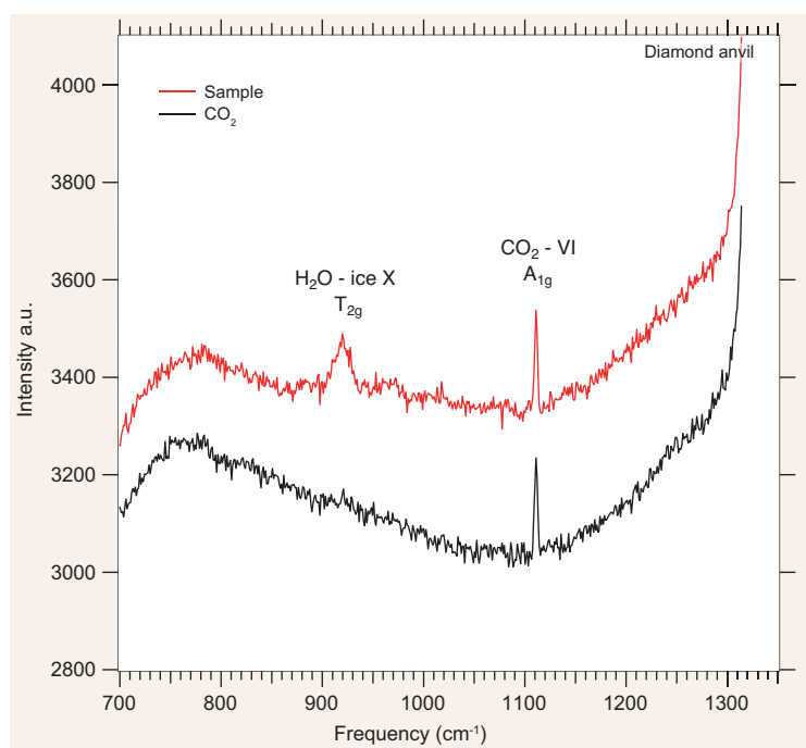
Figure 3. Raman spectra collected after laser heating in the CO 2 area (in black) and sample area (in red).
