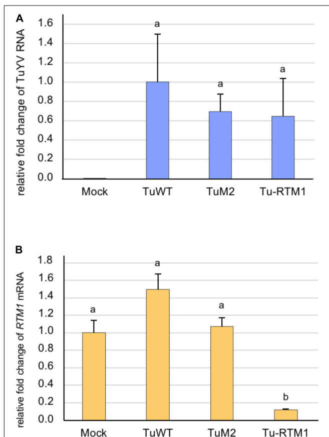
FIGURE 6 | Analysis by real-time RT-PCR of the accumulation of TuYV RNA (A) and RTM1 transcripts (B) in infected A. thaliana Col-0 plants. Plants were either mock-inoculated (mock) or agroinoculated with TuWT, TuM2, or Tu- RTM1 and collected 36 dpi. TuM2 is the parental clone in which the RTM1 sequence was inserted. The bars represent the relative fold-change \pm SE of viral RNA or RTM1 transcripts in upper non-inoculated leaves of individual mock or infected plants. The TuYV value in infected TuWT control plants and the RTM1 value in the mock-inoculated plants were arbitrarily set to 1 as a reference. Statistical analyses were performed using one-way ANOVA following by Tukey's post-hoc test. Different letters above the bars indicate statistically significant differences for RTM1 transcripts (B) ( p -value < 0.05) while the same letters indicate no statistically significant differences (A and B).
