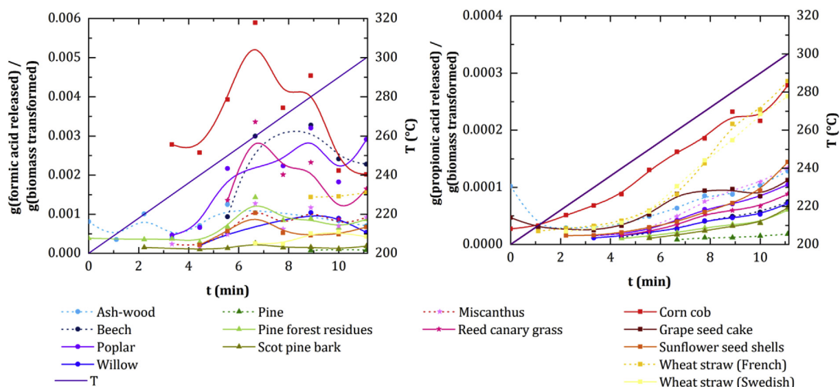
Fig. 7. Production profile of formic acid (left) and propionic acid (right) versus temperature and time obtained for raw biomasses in torrefaction in TGA-GC/MS.
