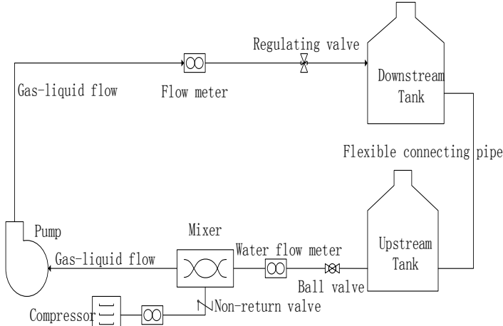
Fig.1 Test rig
