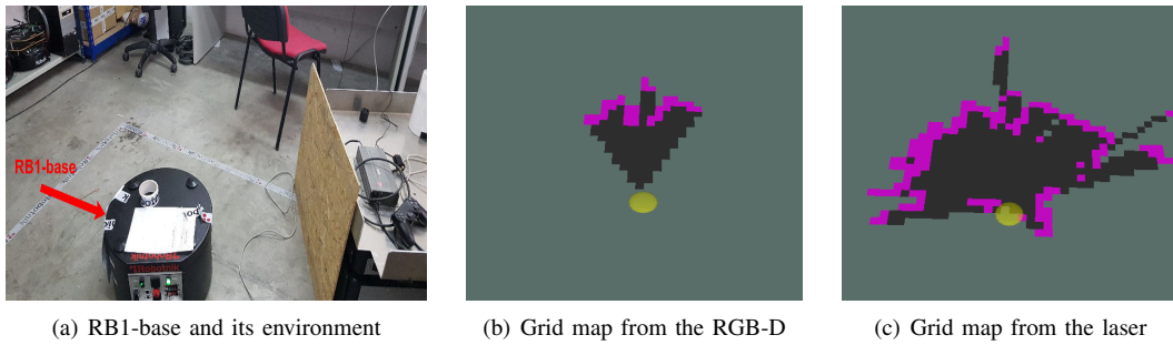
Fig. 1: Robot's environment and the corresponding grid maps from each sensor. Grey, purple and black colors represent unknown, occupied and free respectively. The yellow circle represents the landmark i.e. the robot.
