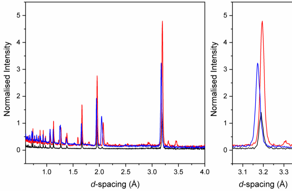
Figure 2. Neutron diffraction patterns of Ge powder collected in single -toroidal SiC-sintered diamond anvils (blue) compared to Co-sintered diamond anvils (black). For comparison, data collected in ZTA anvils (red) are also shown. The load on the anvils is 60 tonnes (in all three data sets), producing a pressure of 7-8-6 GPa. In the right hand panel enlarged region around the (111) reflection from germanium is shown from each anvil for comparison. The accumulation time 1 hr for each pattern, the intensity is normalized to proton current (approximately time).
