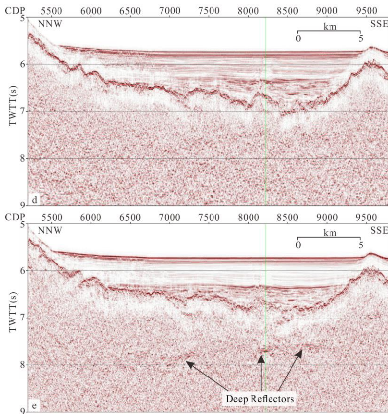
668 Fig.3. The gather of CDP 8218 before peg-leg multiples attenuation (a), after parabolic Radon 669 transform filtering (b) and inner muting (c). Comparison of time-migrated section of profile 670 NH973-1 processed by CNOOC (d) and this study (e). The green lines indicate the location of CDP 671 8218. The vertical exaggeration in (d, e) is 1.5.
