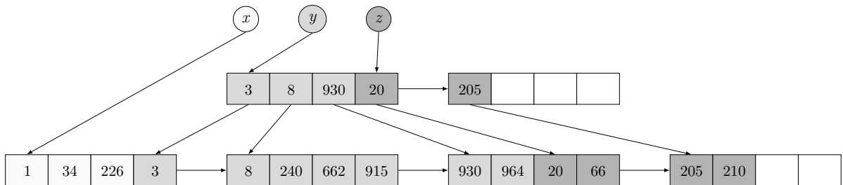
Figure 5: Representation of postings lists
