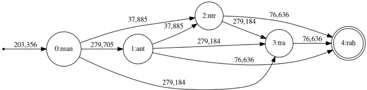
Figure 4: The query string mantrah represented as a directed acyclic graph of trigrams
