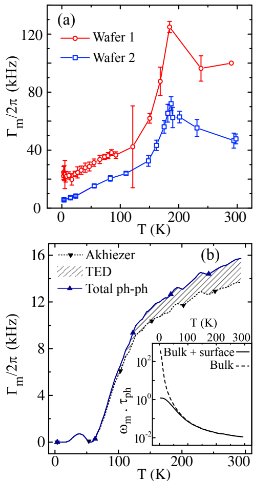
FIG. 2. (a) Measured mechanical dissipation rate as a function of temperature. The two wafers were grown in two distinct MBE chambers. 50 resonators were measured in total, and the here shown results are representative. (b) Modeled mechanical dissipation due to phonon-phonon interactions, for both Akhiezer and TED mechanisms. Note that the damping cancels artificially around 60K with the Grüneisen parameter, as a result of our approximation on \Delta\gamma (see text). Inset: Temperature evolution of the parameter \omega_m\tau_{ph} (see text).
