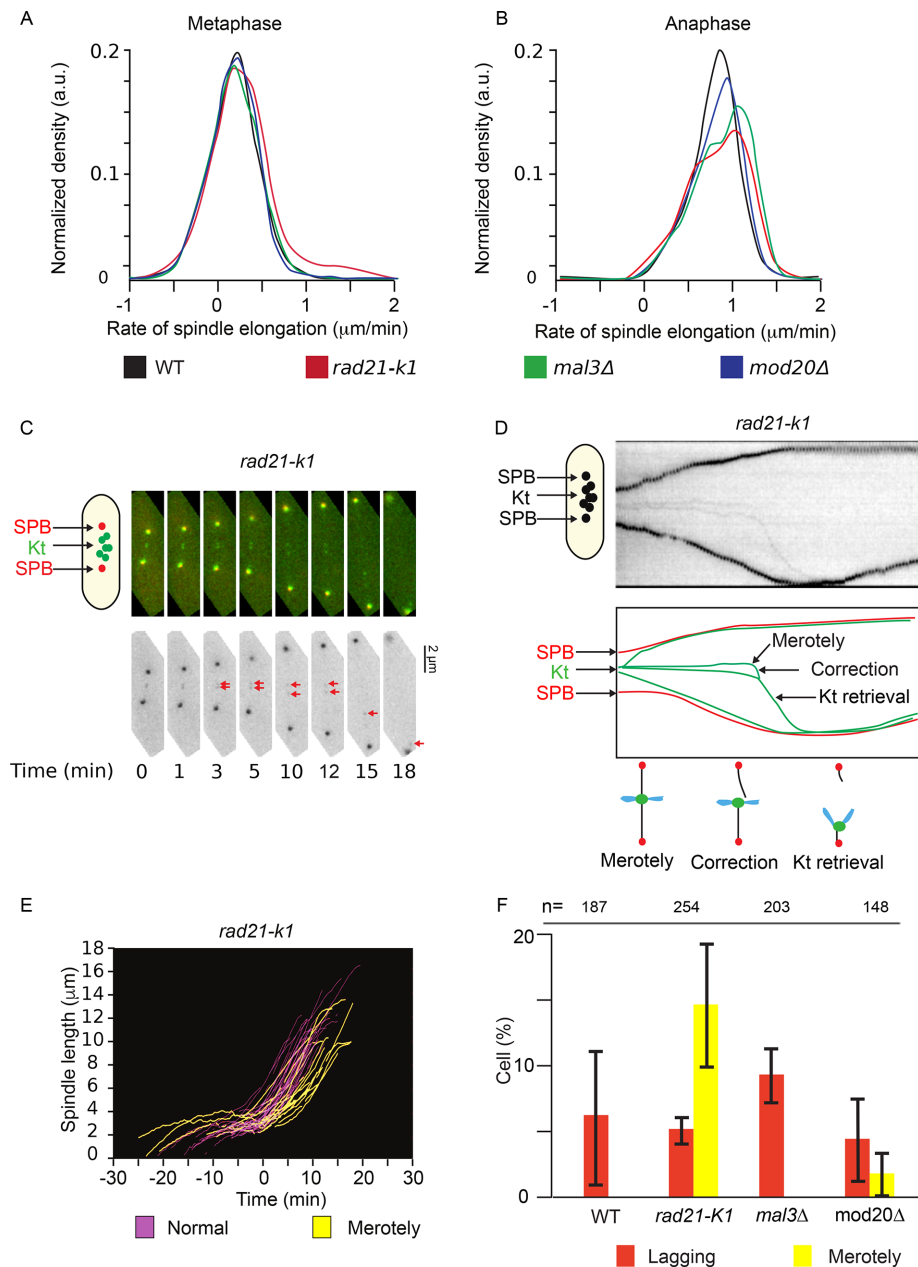
FIGURE 6: Automated detection of lagging kinetochores and merotelic attachment in several genetic backgrounds. (A) Normalized density profiles of spindle elongation speed during metaphase in wild-type (black), rad21-K1 (red), mal3Δ (green), and mod20Δ (blue) cells. (B) Normalized density profiles of spindle elongation speed during anaphase B in wild-type (black), rad21-K1 mutant (red), mal3Δ (green), and mod20Δ (blue) cells. (C) MAARS automatic detection of merotelic kinetochore correction in rad21-K1 cells. Red arrows indicate the position of the merotelic kinetochore. (D) Kymograph representation of the cell shown in C and schematic representation of the correction of the merotelic kinetochore in anaphase. (E) Multiple spindle elongation profiles observed in rad21-K1 cells ( n = 88 ). Spindle elongation profiles in the absence of merotelic attachment are highlighted in pink, and elongation profiles presenting merotelic attachment in anaphase are highlighted in yellow. Time zero corresponds to anaphase onset. (F) Statistical analysis describing the percentages of lagging kinetochores (red) and merotelic kinetochore attachments (yellow) in different cell lines. Error bars correspond to SDs obtained from three independent experiments.
