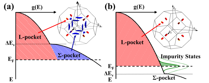
FIG. 1. Illustration of two possible scenarios of valence band filling in \text{Pb}_{1-x}\text{Tl}_x\text{Te} , showing schematic diagrams of the DoS g(E) as a function of energy E , and the FS morphology (insets). (a) The situation in which E_F > \Delta E_v and impurity states play no role. The upper valence band maximum (the L-pocket, red) and the second valence band maximum (the \Sigma -pocket, blue) are both above E_F , giving four degenerate valleys for L-states, and twelve degenerate valleys for \Sigma -states, and an increased DoS for E_F > \Delta E_v where \Delta E_v is the difference in energy between the band maxima. Inset : Calculated FS for E_F > \Delta E_v [15]. (b) The situation in which the \Sigma -band is never populated because resonant impurity states (shown in green) associated with Tl doping occur at E = E_F < \Delta E_v . E_F is pinned by resonant impurity states at an energy E_F < \Delta E_v , leading to an increase in the DoS. Inset : Calculated FS for E_F < \Delta E_v [15]. In this paper we establish that scenario (b) is the correct description for \text{Pb}_{1-x}\text{Tl}_x\text{Te} with x > x_c , with immediate implications for the origin of the anomalous superconductivity observed for this material.
