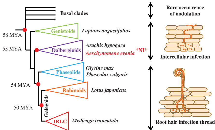
Figure 1. Phylogeny of the Papilionoid lineage and evolution of the symbiotic infection process. The tree is a simplified representation with triangle representing the major clades and the two subclades of the Galegoids: the Robinoids and the plastid DNA inverted repeat-lacking clade (IRLC). Known divergence times are indicated in MYA (million years ago) for some nodes (circles) and notable species are listed for each clade. Symbiotic infection processes encountered in the different clades are reported, excepted for the basal clades for which occurrence of nodulation is restricted to few understudied species. Note that Aeschynomene is the only legume genus where a Nod-independent symbiotic infection process (*NI*) has been reported for several species, including A. evenia . Phylogeny and drawings are adaptations, date estimates and nodulation properties come from previous publications. 2–6
