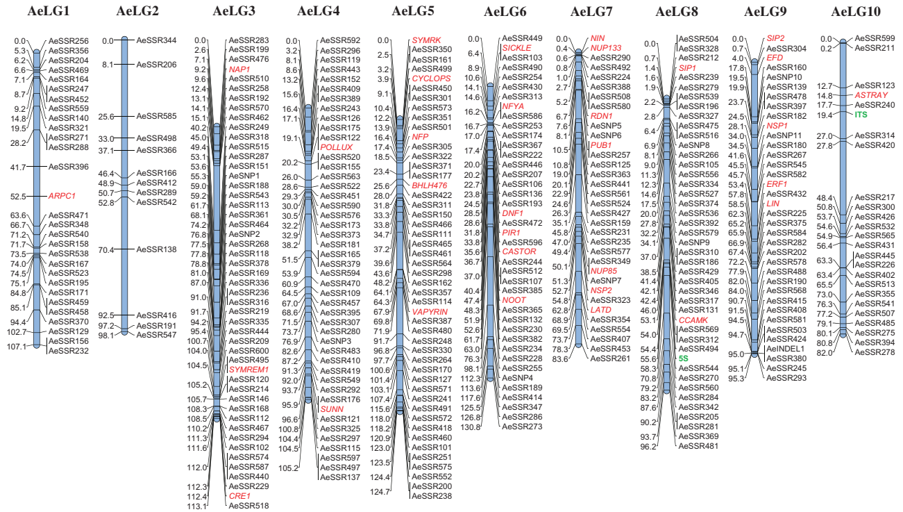
Figure 5. Genetic map of Aeschynomene evenia . The genetic map based on F 2 mapping population CIAT22838 × CIAT8232 is comprised of 364 gene based markers including SSR, INDEL and SNP (KASP) markers. The ten linkage groups are designated as AeLG1-AeLG10. The code to the right of the linkage groups refers to the marker or symbiotic gene name. The numbers to the left of the linkage groups refers to the genetic distances (Kosambi cM) from the top.
