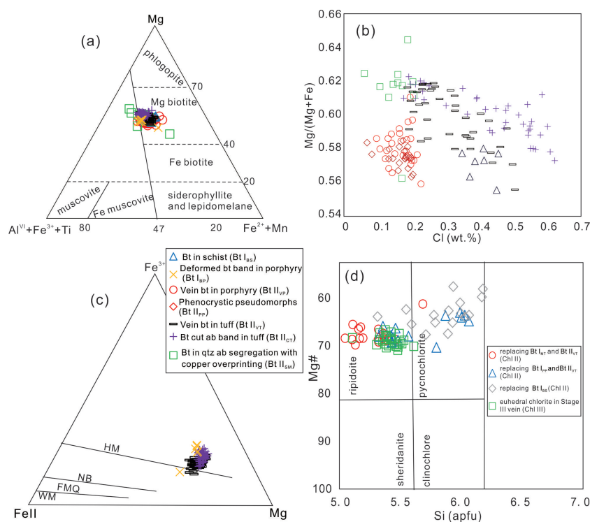
Figure 8. (a) Mg – ( \text{Al}^{\text{VI}} + \text{Fe}^{3+} + \text{Ti} ) – ( \text{Fe}^{2+} + \text{Mn} ) ternary diagram for biotite of the Tongkuangyu Cu deposit, North China Craton; (b) A \text{Mg}/(\text{Mg} + \text{Fe}) versus Cl plot for biotite; (c) \text{Fe}^{3+} – \text{Fe}^{2+} – Mg ternary diagram for oxygen fugacity estimation of biotite; (d) A plot of Mg# versus Si atoms for classification of chlorite at Tongkuangyu. MH: Magnetite-hematite buffer, NB: Nickel-bunsenite; FMQ: Fayalite-magnetite-quartz; WM: Wüstite-magnetite; \text{Mg}\# = \text{Mg}/(\text{Mg} + \text{Fe}) .
