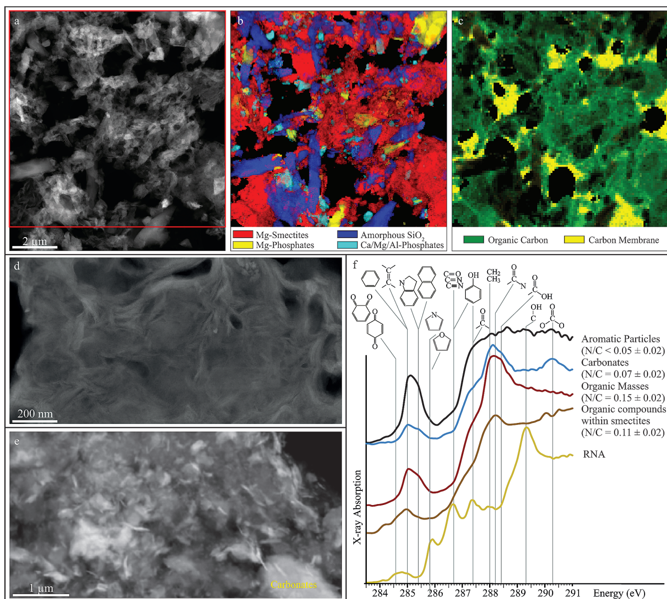
Figure 1 STEM and STXM characterisation of the experimental residues. (a) STEM image of the residues of experiments conducted under \text{CO}_2 at 200 °C in the presence of Mg-smectites and RNA. (b,c) Maps of minerals and organic compounds (same area as a ). (d) STEM images of Mg-smectites. (e) STEM image of sub-micrometric minerals embedded in organic masses. (f) XANES spectra of organic compounds encountered in the residues. The spectrum of RNA is shown for comparison.
