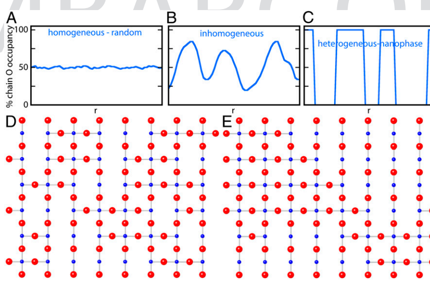
Fig. 4. Conceptual depictions of O vacancies in Sr_2CuO_{3.3} . The a -oriented -Cu-O- chain occupancy distribution for: (A) a random, homogeneous distribution caused by no cooperativity between the O atoms; (B) a moderate tendency for clustering resulting in an inhomogeneous distribution; (C) a strong tendency for clustering causing nanophase separation and a heterogeneous structure composed of domains below the diffraction limit in size consisting of either CuO_2 planes or -Cu-O- chains. (D) The corresponding structure of A. (E) The corresponding structure of C.
