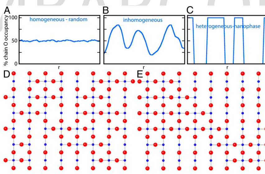
Fig. 4. Conceptual depictions of O vacancies in \text{Sr}_2\text{CuO}_{3.3} . The a -oriented -Cu-O- chain occupancy distribution for: (A) a random, homogeneous distribution caused by no cooperation between the O atoms; (B) a moderate tendency for clustering resulting in an inhomogeneous distribution; (C) a strong tendency for clustering causing nanophase separation and a heterogeneous structure composed of domains below the diffraction limit in size consisting of either \text{CuO}_2 planes or -Cu-O- chains. (D) The corresponding structure of A. (E) The corresponding structure of C.
