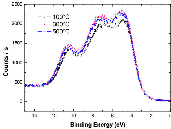
FIG. 2: X-ray photoemission valence bands spectra of the Yb: \text{SnO}_2 thin films as a function of the deposition temperature.
