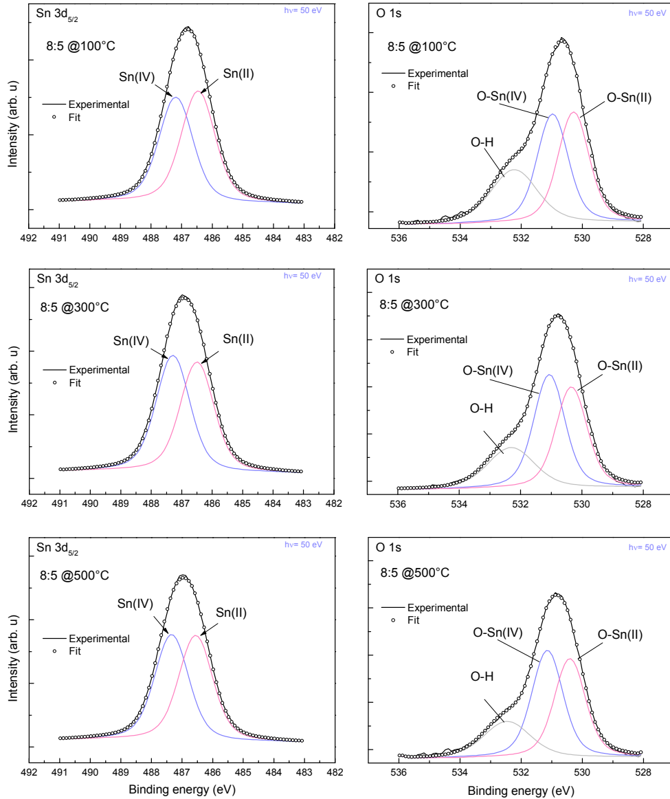
FIG. 3: X-ray photoemission spectra of the 3d_{5/2} and 1s core levels of Sn and O, respectively, recorded on Yb-doped \text{SnO}_2 films grown at different deposition temperatures.
