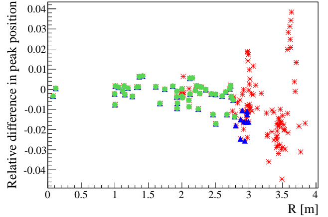
FIG. 49. The relative difference \frac{N_h(MC) - N_h(data)}{N_h(data)} as a function of the radial position R of the ^{214}\text{Po} \alpha peak from the radon calibration source. Blue triangles: ^7\text{Be} - \nu FV, green circles: pep - \nu FV, red stars: outside both FVs.
