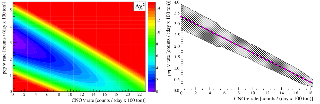
FIG. 75. Correlation between the \text{pep} and CNO neutrino rates. Left: \Delta\chi^2 map obtained from a likelihood-ratio test between the likelihood of the best-fit result and the maximum likelihood returned by the fit when \text{pep} and CNO neutrino interaction rates are fixed to different values. The right column gives the colors corresponding to \Delta\chi^2 values; note that the same red color has been used to plot all \Delta\chi^2 \geq 14 values to allow to visualize color variations in the relevant region of the plot. The numerical values of this map are given in Table XXIII. The plot has been obtained using N_{pe}^d energy estimator; we get similar and consistent numbers using the N_h variable. Right: \text{pep-}\nu interaction rate returned by the fit for different (fixed) CNO neutrino interaction rates. The shaded area is the statistical uncertainty.
