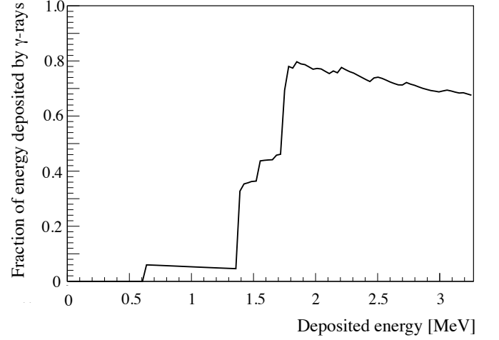
FIG. 44. Average fraction of the energy deposited by ^{214}\text{Bi} decays in the form of \gamma -rays. For deposited energy below 1400 keV, only less than 5% of the energy is due to \gamma -rays. Therefore, low-energy ^{214}\text{Bi} decays are a sample of mostly pure \beta^- decays.
