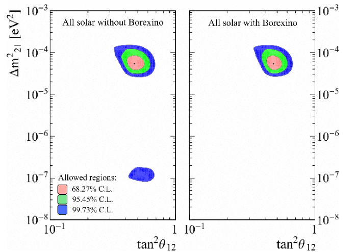
FIG. 80. Allowed regions (NDF = 3) of the space of parameters at 68.27% C.L. (pink), 95.45% C.L. (green), and 99.73% C.L. (blue) by the solar-without Borexino (left panel) and solar-with Borexino (right panel) data set.
