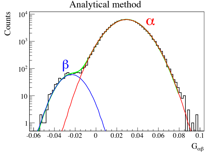
FIG. 36. Example of \alpha - \beta statistical subtraction with the analytical method for events in the energy range 200 < N_{pe}^d < 205 . The blue and red lines show the individual Gaussian fits to the Gatti parameter distributions for the \beta and \alpha components, respectively, while the green line is the total fit.
