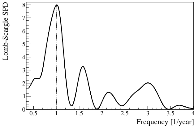
FIG. 66. Lomb-Scargle periodogram for the red data points marked (a) in Fig. 65 after the subtraction of the exponential trend due to the ^{210}\text{Bi} contamination. The Spectral Power Density at 1-year is 7.961, as indicated by the vertical line.
