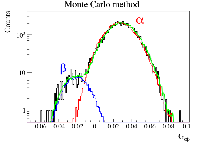
FIG. 37. Example of \alpha - \beta statistical subtraction with the Monte Carlo method for events in the energy range 168 < N_h < 170 . The plot shows the Gatti parameter of the data (black) and the fit (green) aiming to separate the \alpha (red) and \beta (blue) contributions. In comparison to analytical method demonstrated in Fig. 36, the blue \beta and \alpha shapes are Monte Carlo shapes which are not Gaussian. Details in text.
