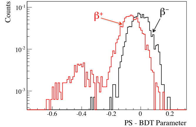
FIG. 45. Distributions of the PS-BDT parameter for the test samples of \beta^- (black) and \beta^+ (red) events as described in the text.
