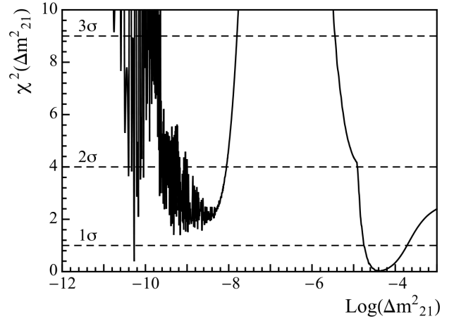
FIG. 79. The \chi^2 -profile of the \Delta m_{21}^2 parameter in the Borexino results analysis. The dashed lines indicate the 1\sigma [ \chi^2(\Delta m_{21}^2) = 1 ], 2\sigma [ \chi^2(\Delta m_{21}^2) = 4 ], and 3\sigma [ \chi^2(\Delta m_{21}^2) = 9 ] levels. The MSW-LOW region ( 10^{-8} \text{ eV}^2 < \Delta m_{21}^2 < 10^{-6} \text{ eV}^2 ) is ruled out at more than 8.5\sigma .
