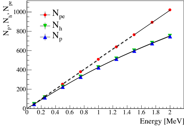
FIG. 50. The energy estimators N_p , N_h , and N_{pe} versus energy for \beta events uniformly generated in the {}^7\text{Be} -FV as obtained with the Monte Carlo simulation.
