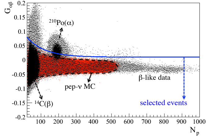
FIG. 35. The distribution of the Gatti G_{\alpha\beta} parameter as a function of energy ( N_p variable). The continuous (blue) line shows the energy dependent cut; it removes all the events with G_{\alpha\beta} above the line. The (red) points enclosed within the dashed line show the G_{\alpha\beta} distribution for MC-simulated pep-\nu 's; these events are an example of true \beta events with a spectrum extending over a sufficiently large energy range. The \beta events are not affected by this cut, while, on the contrary, this cut removes a large fraction of the \alpha events, as those from the {}^{210}\text{Po} decay.
