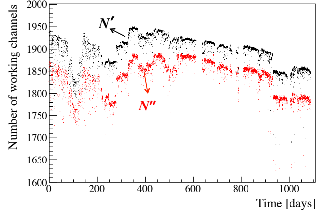
FIG. 10. The number N' (black) and N'' (red) of available channels for the computation of N_h / N_p and N_{pe} energy estimators, respectively, as a function of time starting from May 16 th , 2007 (day 0). The slow decrease is due to the PMT mortality, while the sudden changes are due to the failure/repair of the electronics.
