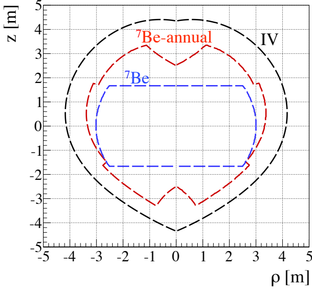
FIG. 17. \rho - z projection of the IV as of May 3 rd , 2009 (black). The blue curve shows the shape of the 75 ton FV used for the measurement of the {}^7\text{Be} - \nu interaction rate. The red curve illustrates the profile of the FV used for the {}^7\text{Be} - \nu annual modulation analysis.
