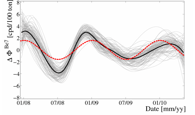
FIG. 69. Set of 100 intrinsic mode functions \text{IMF}_8 extracted after the addition of dithering (grey lines). The black-solid line is their average and the dashed-red line is the annual modulation from Eq. 84. The number of the IMF is the expected one for the annual frequency of \nu_{\text{year}} = 0.00274 [d^{-1}] .
