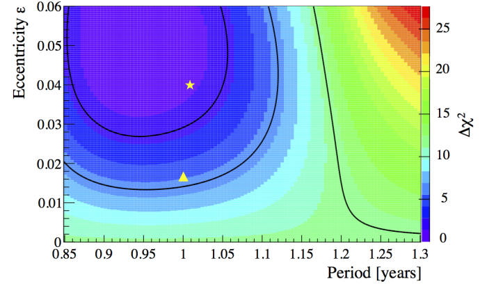
FIG. 64. The results obtained via the fit of the rate-versus-time distribution shown in Fig. 63: a \Delta\chi^2 ( \Delta\chi_R^2 = \chi_{R_{min}}^2 - \chi_{R_{xy}}^2 ) map (vertical axis) as a function of eccentricity \varepsilon and period. The yellow star indicates the best-fit results, while the yellow triangle the expected values. Confidence contours of 1, 2, and 3\sigma are indicated with black solid lines.
