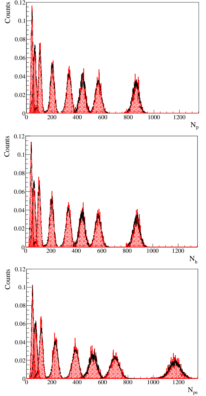
FIG. 47. Energy spectra ( N_p , N_h , and N_{pe}^d variables) of the calibration sources placed in the detector's center: measured data (black lines) versus the Monte Carlo simulation (areas dashed with red lines). The peaks represent (from the left to the right) the total \gamma decay energy of ^{57}\text{Co} , ^{139}\text{Ce} , ^{203}\text{Hg} , ^{85}\text{Sr} , ^{54}\text{Mn} , ^{65}\text{Zn} , ^{40}\text{K} , and ^{60}\text{Co} .
