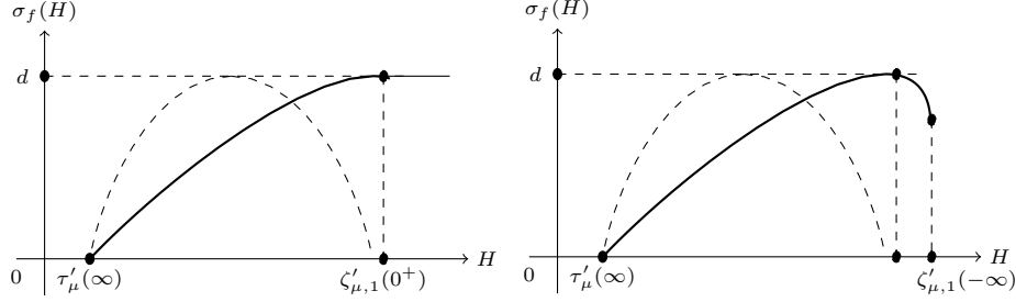
FIGURE 4. Here we take p = 1 . Left: Upper bound for the multifractal spectrum of every f \in B_q^{\mu,1}(\mathbb{R}^d) . Right: Multifractal spectrum of a typical function in \tilde{B}_q^{\mu,1}(\mathbb{R}^d) . The dashed graph represents the (initial) multifractal spectrum of \mu . When p = \infty , the multifractal spectrum of typical f \in \tilde{B}_q^{\mu,\infty}(\mathbb{R}^d) coincides with that of \mu .
