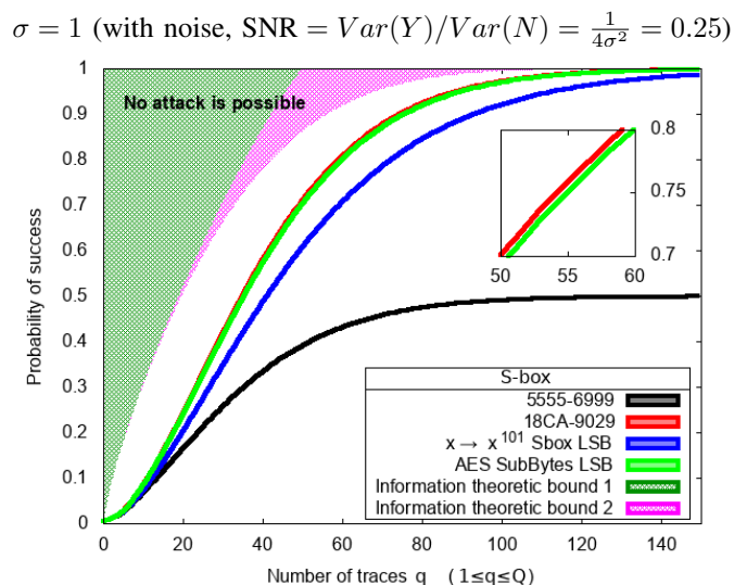
Fig. 4. Success rate of attack with noise for various S-boxes and attack bounds, with similar inset magnification as in Fig. 3.
