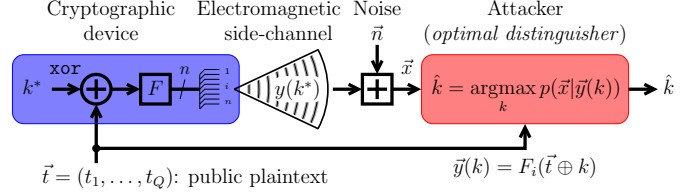
Fig. 1. Attack setup on the leakage function y = f(t \oplus k^*) , where t is one known plaintext, k^* is the secret key, F is the substitution box and i is the leaking coordinate of F (hence f = F_i )
