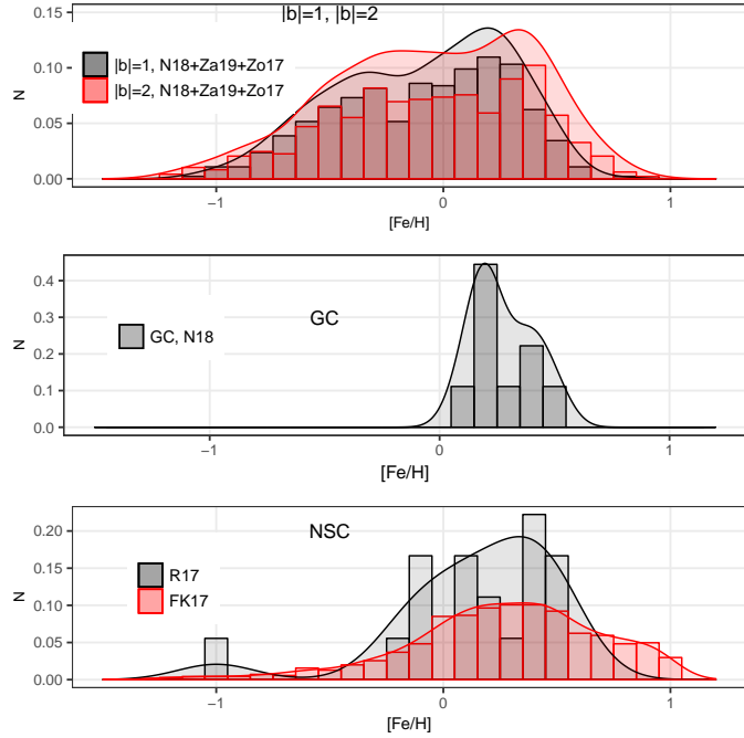
Fig. 3. Normalized Metallicity Distribution Function of M giants in inner two degrees. Upper panel: distributions at |b| = 1 deg and |b| = 2 deg from Zol17, N18, and Za19. Middle panel: same for the GC field from N18, and lower panel: for the NSC from FK17 and R17. A kernel density estimation with a bin size of 0.1 dex is also overplotted as a solid line.
