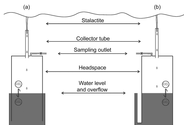
Figure 3. Schematic of the two water–air equilibrators used for the measuring of drip water CO 2 : Type A (a) and Type B (b).
