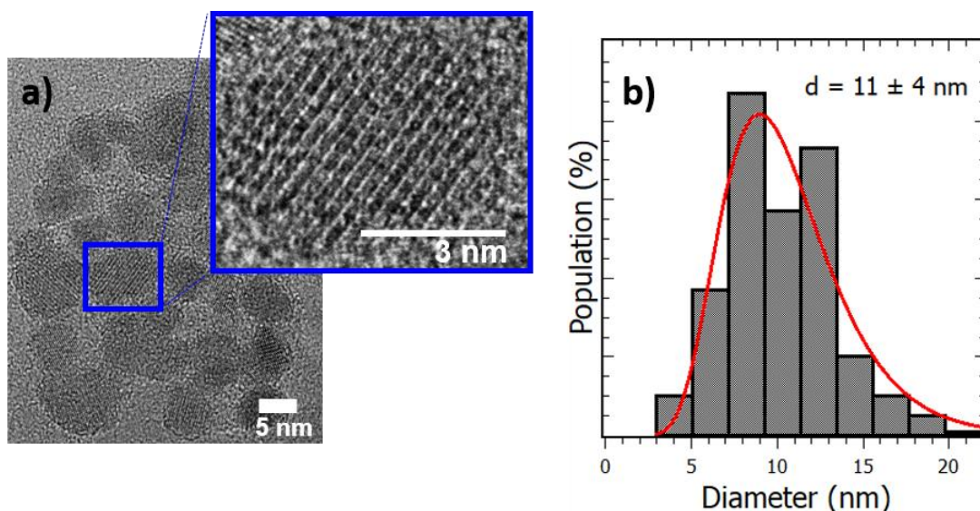
Figure 1. a) Representative HRTEM image with a magnification in inset and b) size histogram of the magnetic NPs with the mean value and the variance of the distribution.
