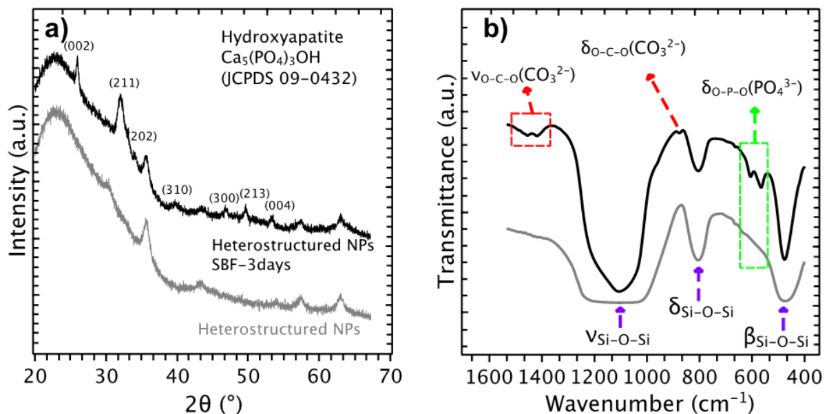
Figure 8. a) XRD profiles and b) FTIR spectra of heterostructured NPs before (grey, bottom) and after (black, up) 3 days of immersion in SBF.
