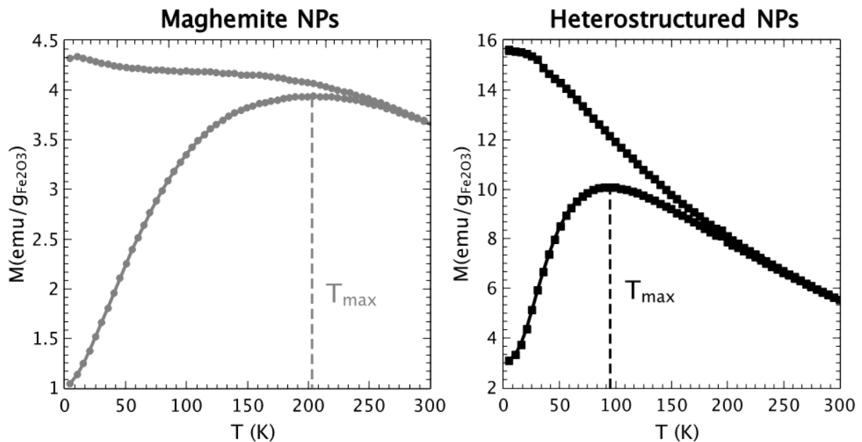
Figure 5. ZFC-FC magnetization curves of maghemite and heterostructured nanoparticles recorded at 25 G.
