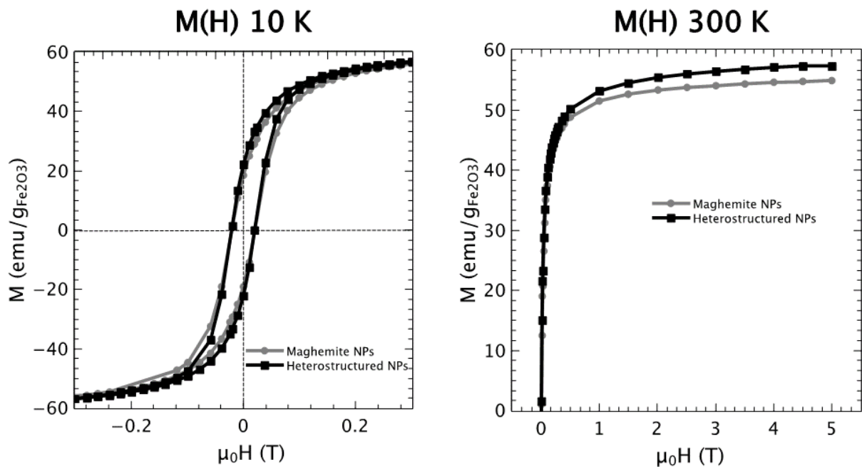
Figure 4. M(H) curves of maghemite (grey, circles) and heterostructured (black, square) NPs at 10 K and 300 K.
