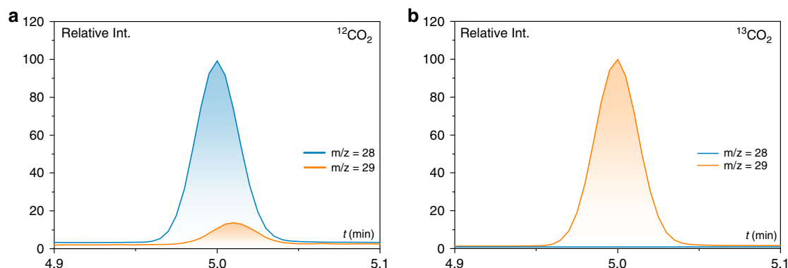
Fig. 6 GC/MS chromatograms at the retention time of carbon monoxide. Specific traces of m/z = 28 value (blue) and m/z = 29 value (orange) after 2 h of electrolysis at illuminated Co-qPyH|f-TiO 2 |CIGS ( E_{\text{bias}} = -0.06 V vs. RHE), in 0.1 M KHCO 3 electrolyte saturated with 12 CO 2 (a) and 13 CO 2 (b).
